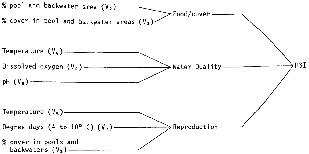
Figure 1. Tree diagram illustrating relationships between model variables, components (life requisites) and HSI for the riverine yellow perch model.
