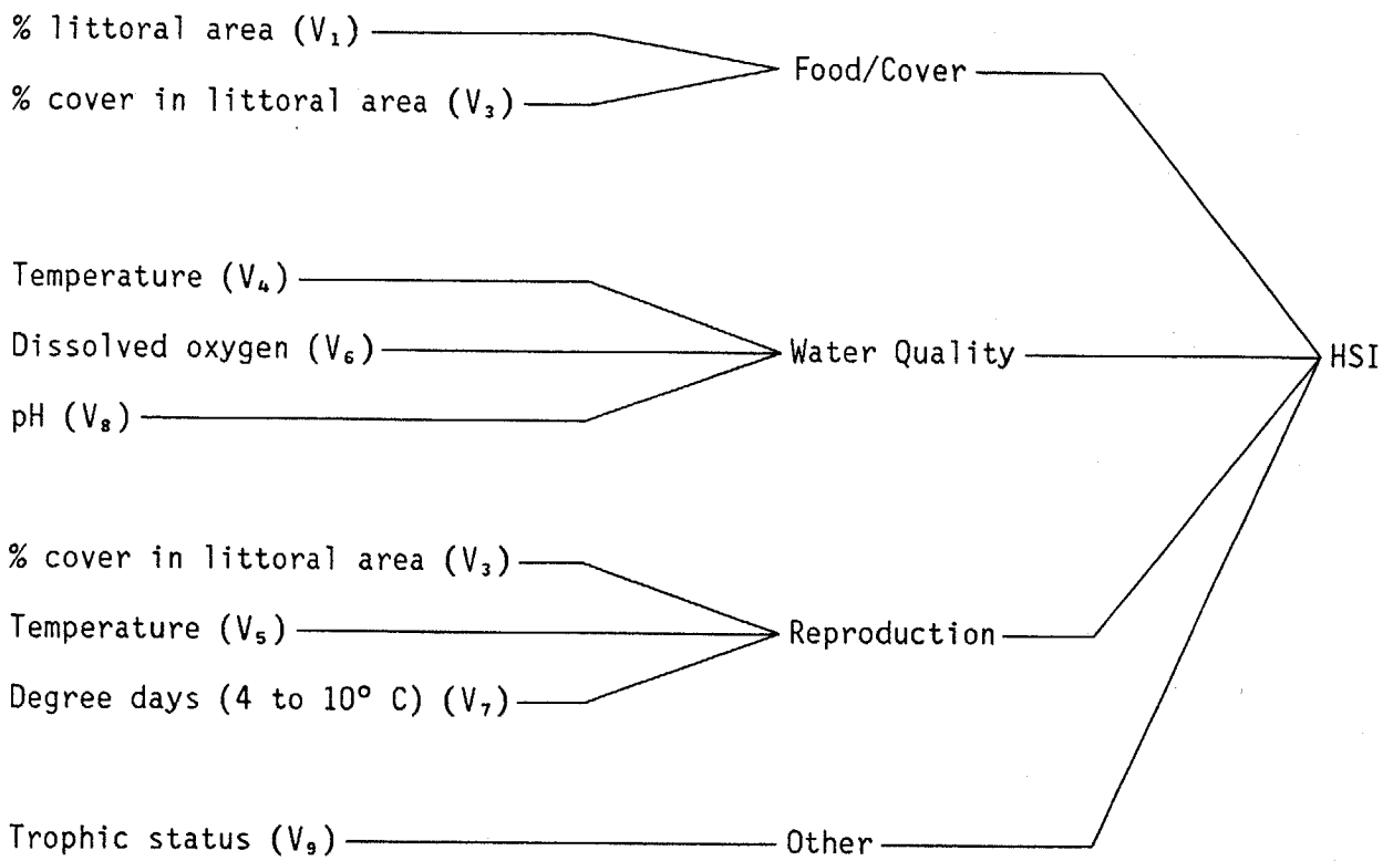
Figure 2. Tree diagram illustrating relationships between model variables, components (life requisites) and HSI for the lacustrine yellow perch model.
