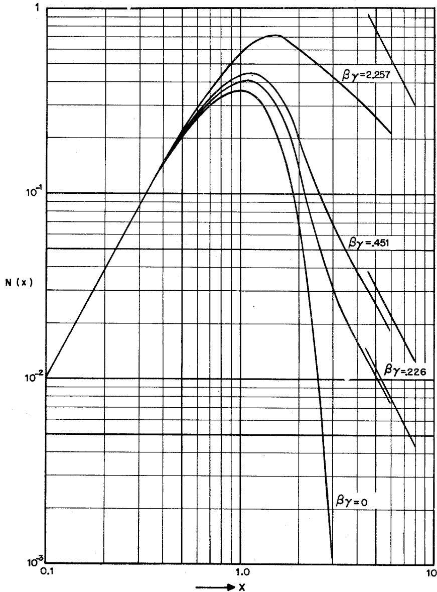
Figure 1. Graphs showing N(x) for \beta\gamma = 0, 0.226, 0.451, and 2.257, and its asymptotic behavior for large X for \beta\gamma = 0.226, 0.451, and 2.257. x is proportional to the velocity, X = 1 corresponding to kT.
