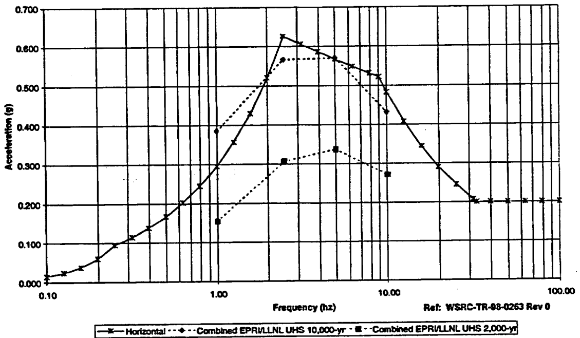
Comparison of 0.2g Regulatory Guide 1.60 Response Spectra (Horizontal 5% Damping) to Soil Surface UHS at Four Spectral Frequencies
