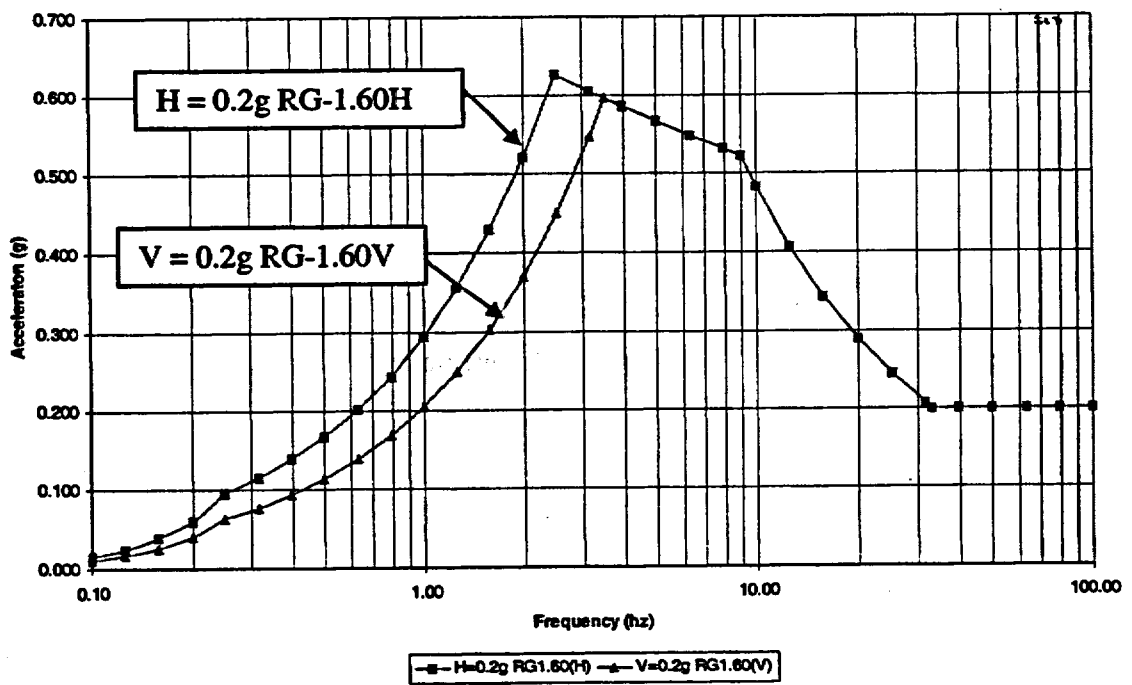
MFFF Design Earthquake Response Spectra (5% Damping)
