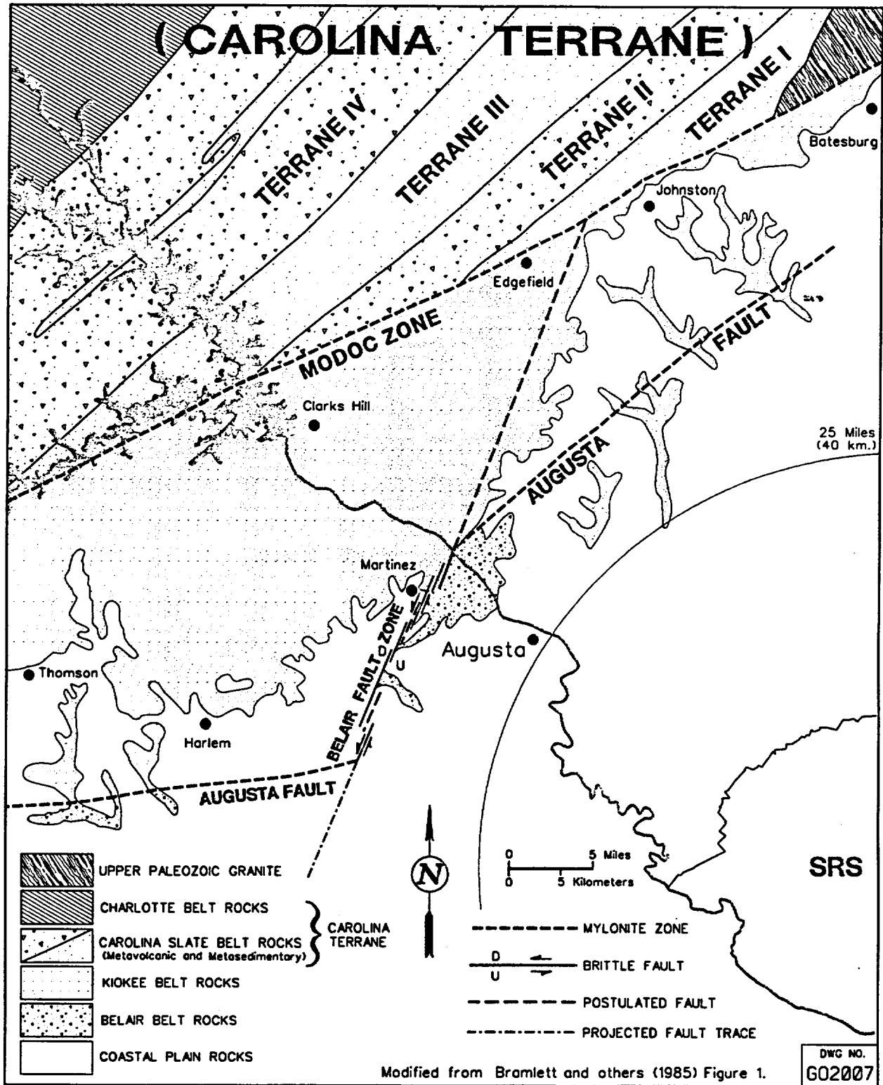
Figure 1.3.6-10. Carolina Terrane
