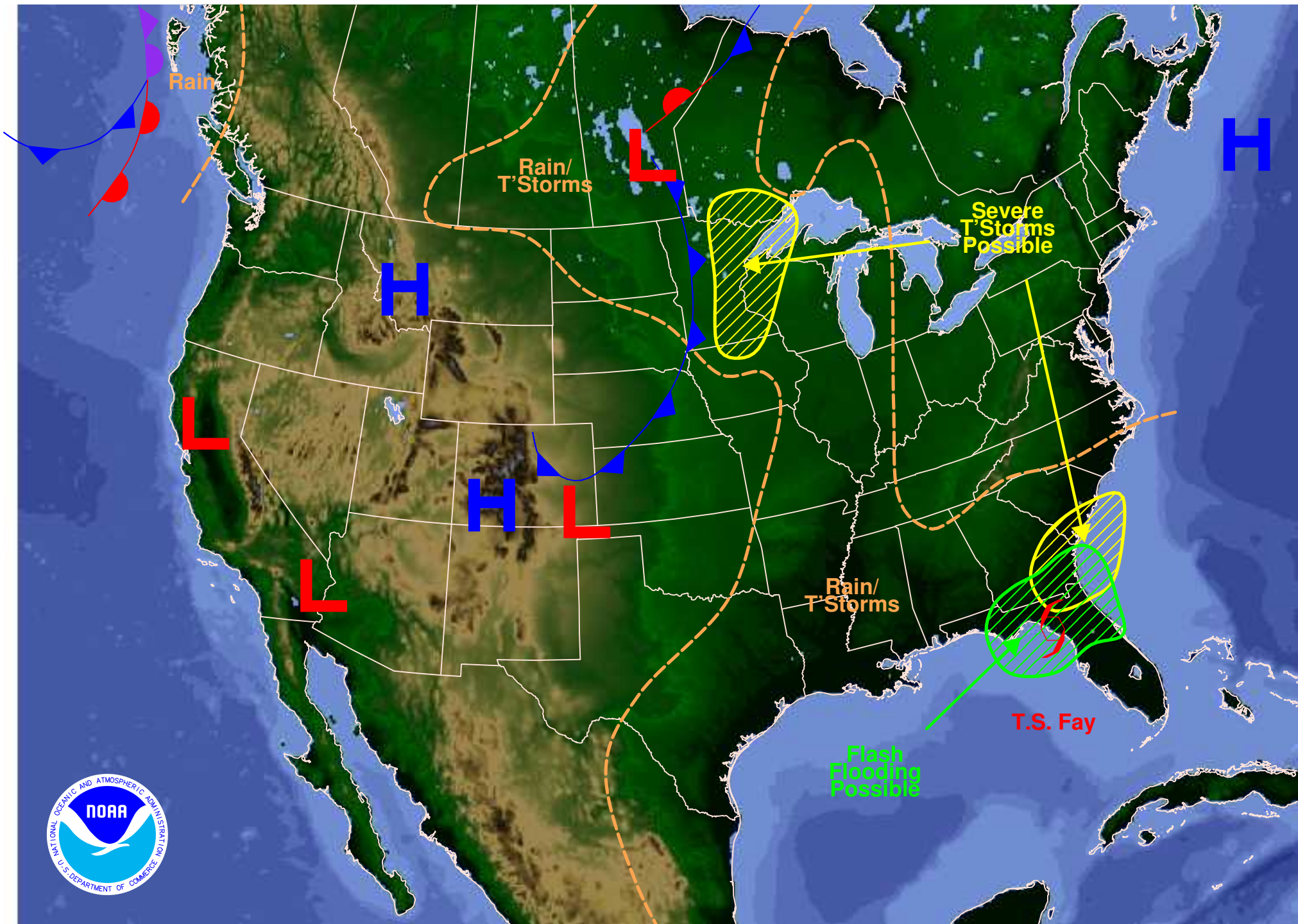
Weather Forecast for Friday, August 22, 2008 DOC/NOAA/NWS/NCEP/Hydrometeorological Prediction Center Prepared by Fracasso based on HPC, SPC, and TPC forecasts.
