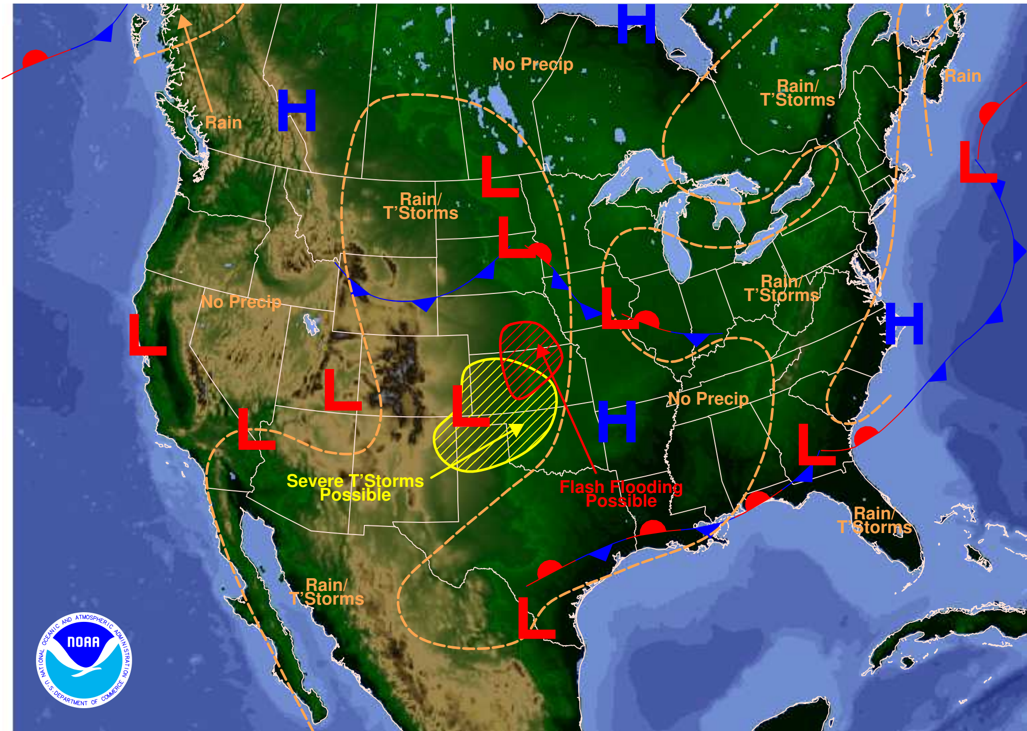
Weather Forecast for Thursday, August 14, 2008 DOC/NOAA/NWS/NCEP/Hydrometeorological Prediction Center Prepared by Kost based on HPC, SPC, and TPC forecasts.
