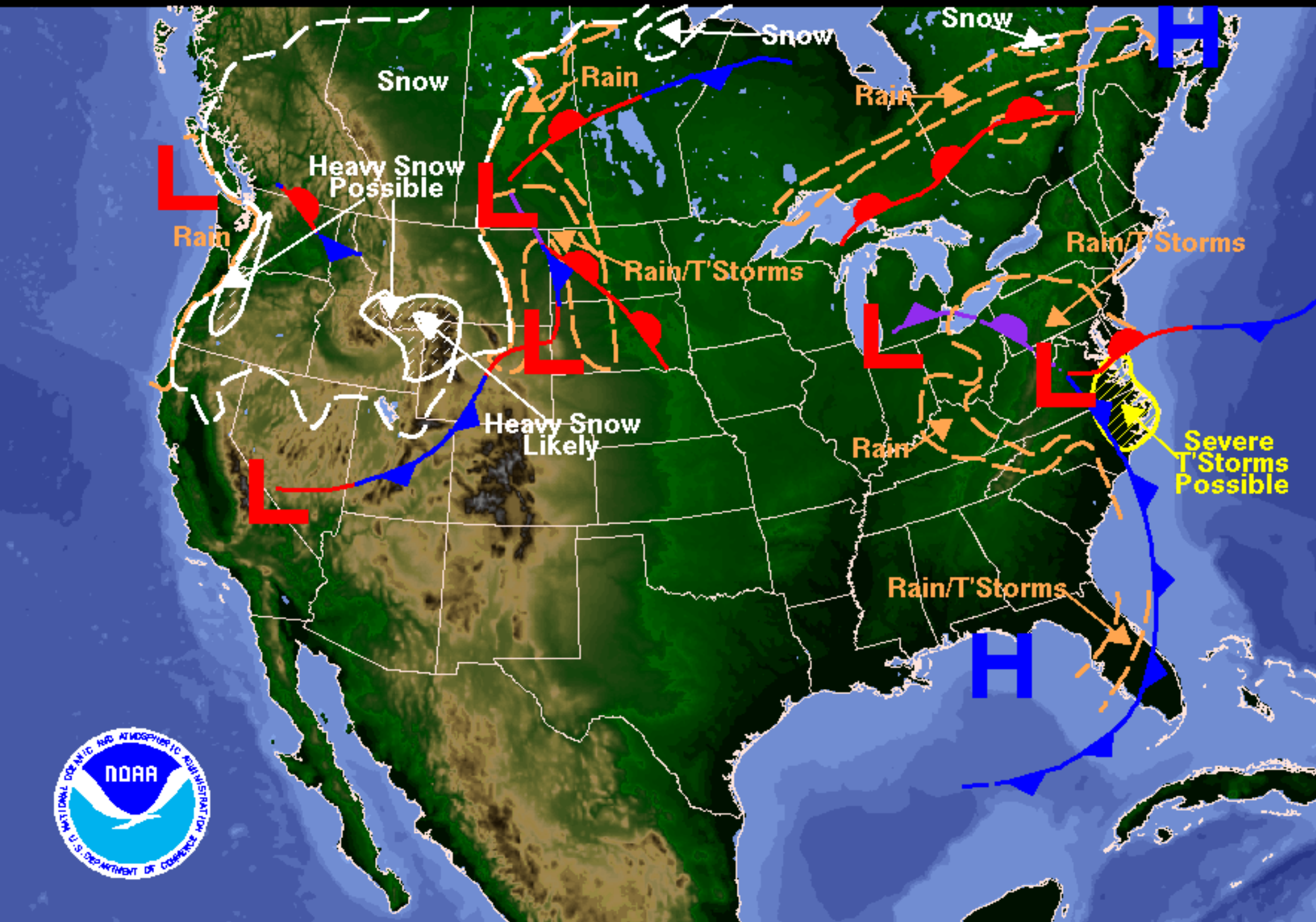
Weather Forecast for Sunday, April 20, 2008 DOC/NOAA/NWS/NCEP/Hydrometeorological Prediction Center Prepared by Collins based on HPC, SPC, and TPC forecasts.
