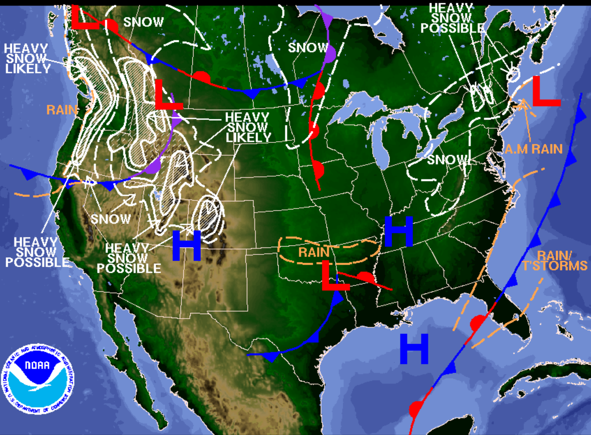
Weather Forecast for Thursday, February 07, 2008 DOC/NOAA/NWS/NCEP/Hydrometeorological Prediction Center Prepared by oravec based on HPC, SPC, and TPC forecasts.
