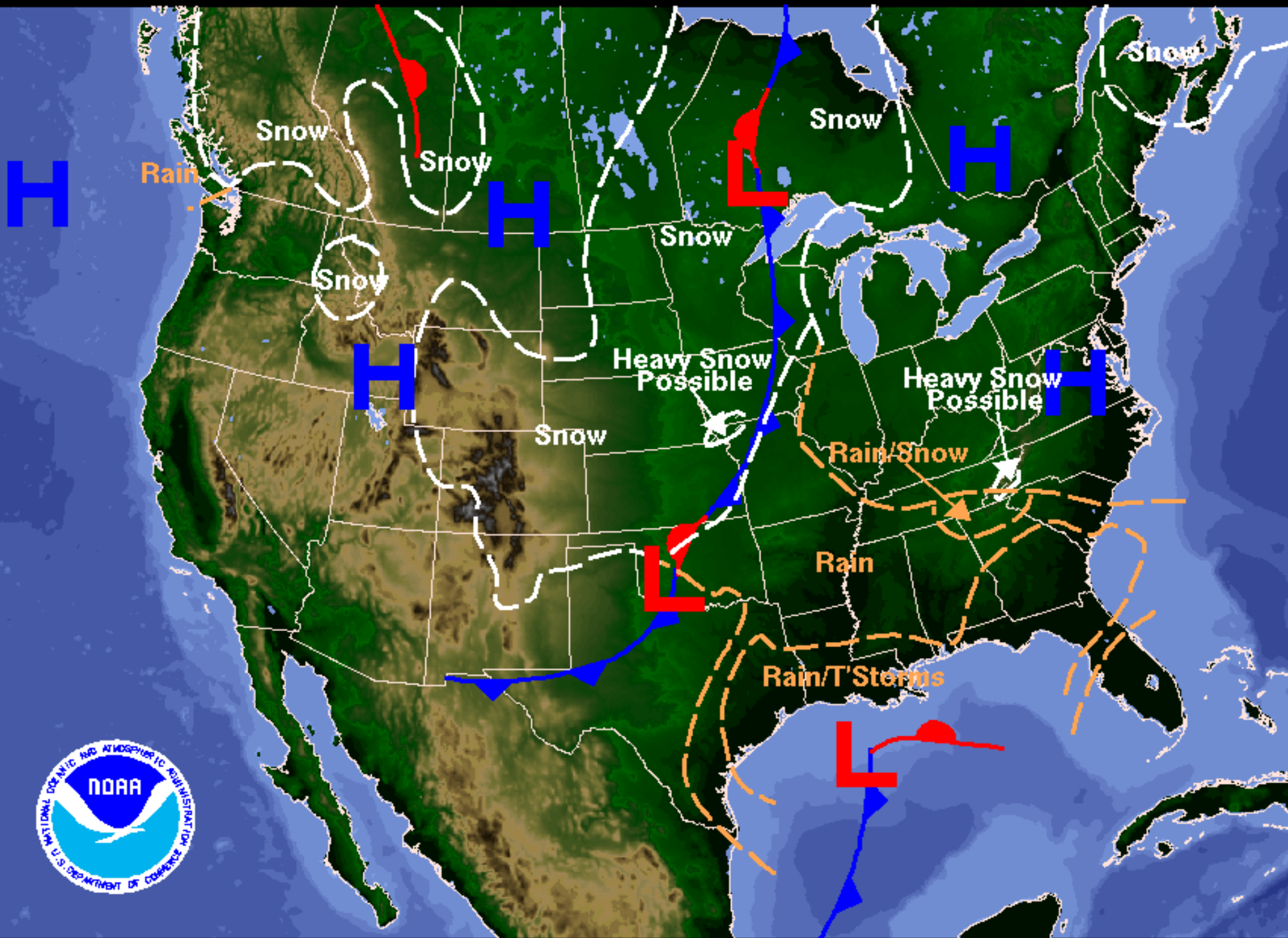
Weather Forecast for Wednesday, January 16, 2008 DOC/NOAA/NWS/NCEP/Hydrometeorological Prediction Center Prepared by Collins based on HPC, SPC, and TPC forecasts.
