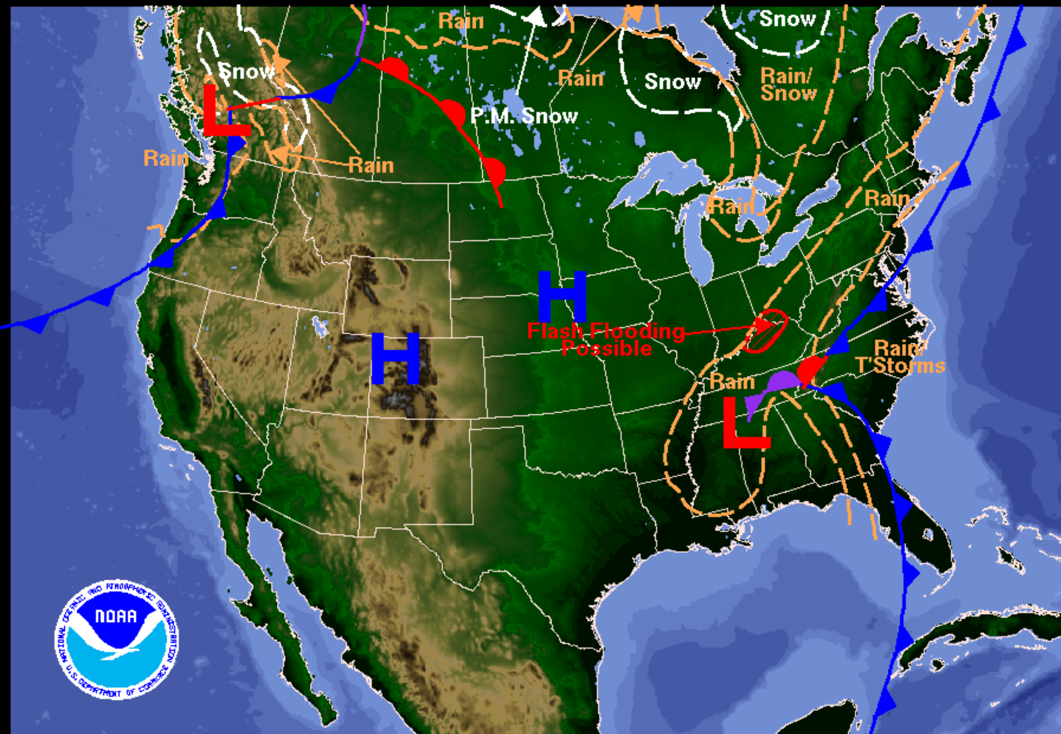
Weather Forecast for Wednesday, October 24, 2007 DOC/NOAA/NWS/NCEP/Hydrometeorological Prediction Center Prepared by Rubin-Oster based on HPC, SPC, and TPC forecasts.
