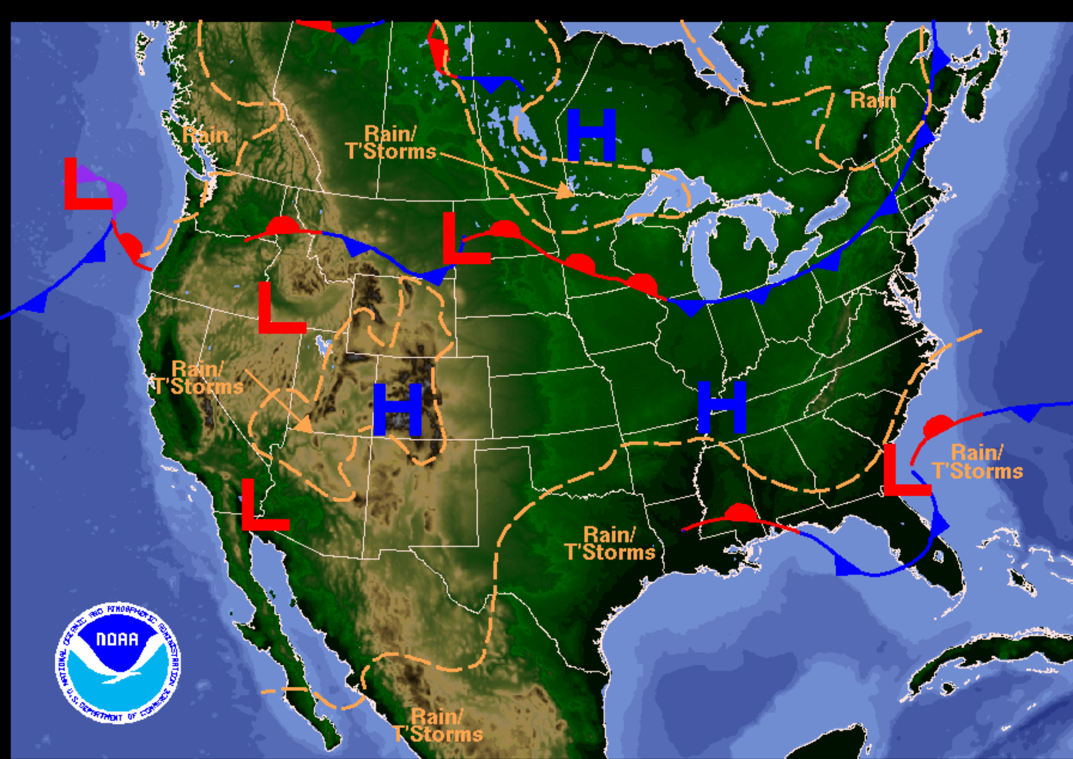
Weather Forecast for Monday, September 03, 2007 DOC/NOAA/NWS/NCEP/Hydrometeorological Prediction Center Prepared by Otto based on HPC, SPC, and TPC forecasts.
