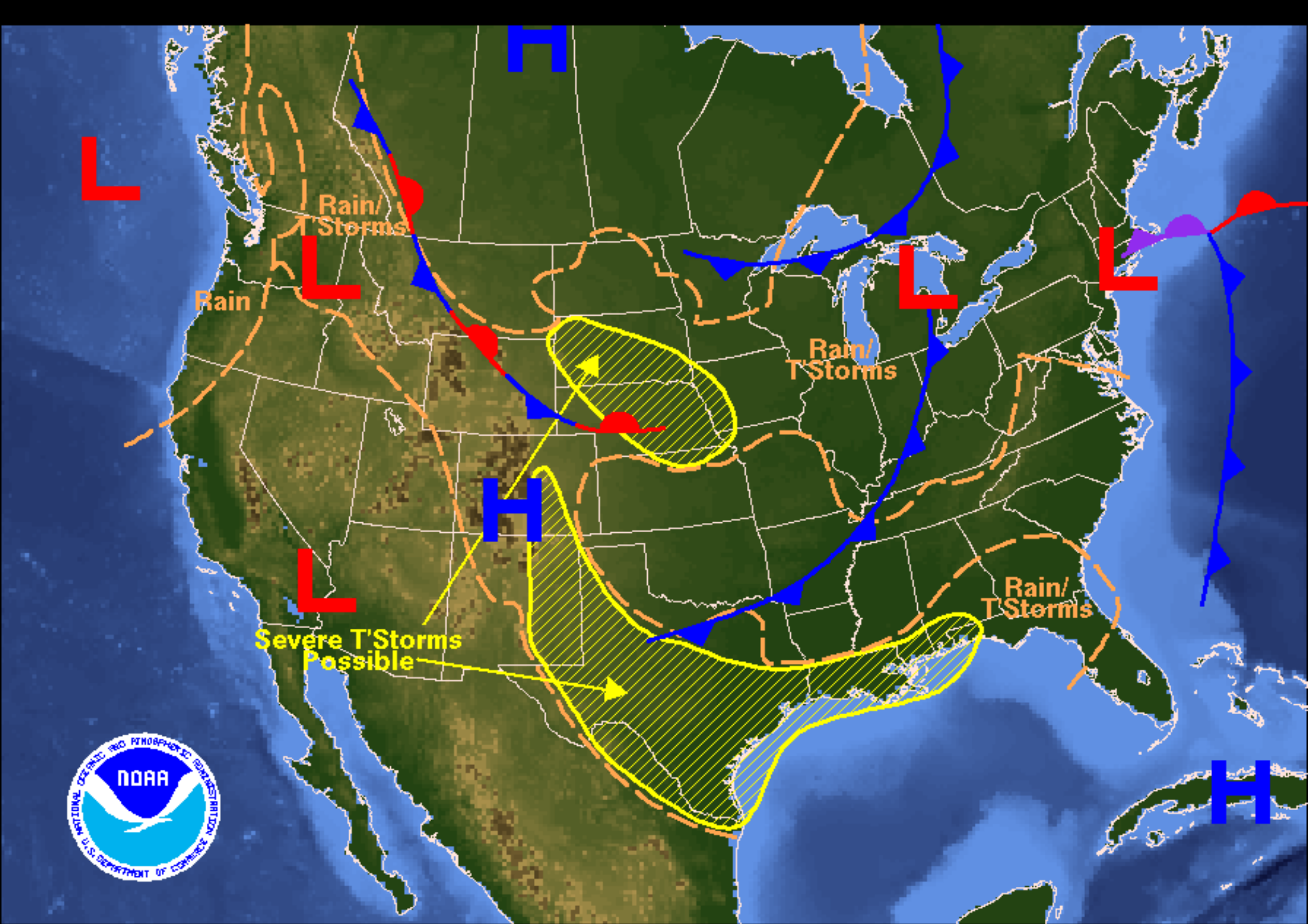
Weather Forecast for Monday, June 04, 2007 DOC/NOAA/NWS/NCEP/Hydrometeorological Prediction Center Prepared by Rubin-Oster based on HPC, SPC, and TPC forecasts.
