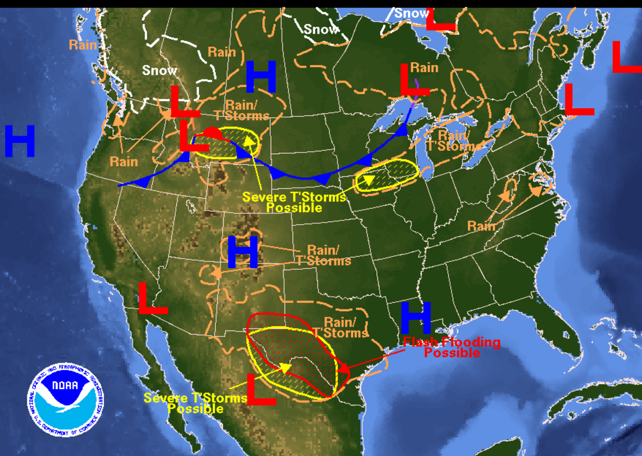
Weather Forecast for Sunday, April 29, 2007 DOC/NOAA/NWS/NCEP/Hydrometeorological Prediction Center Prepared by Rubin-Oster based on HPC, SPC, and TPC forecasts.
