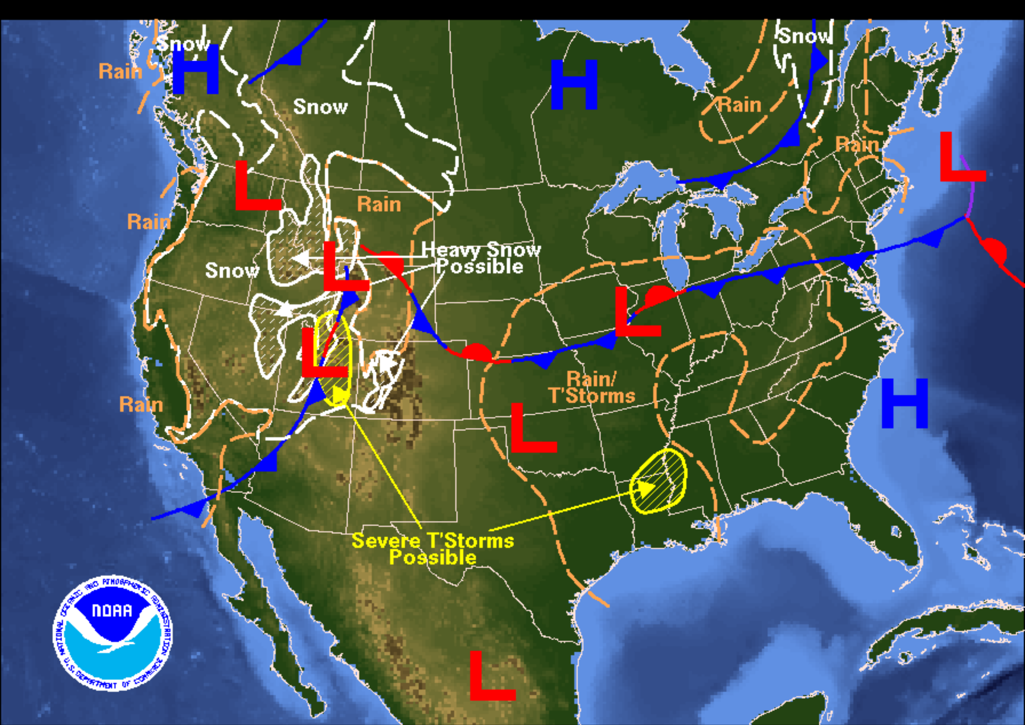
Weather Forecast for Tuesday, March 27, 2007 DOC/NOAA/NWS/NCEP/Hydrometeorological Prediction Center Prepared by Rubin-Oster based on HPC, SPC, and TPC forecasts.
