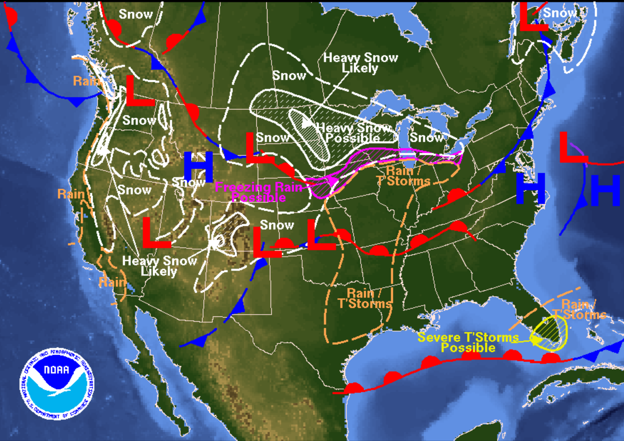
Weather Forecast for Wednesday, February 28, 2007 DOC/NOAA/NWS/NCEP/Hydrometeorological Prediction Center Prepared by Kong based on HPC, SPC, and TPC forecasts.
