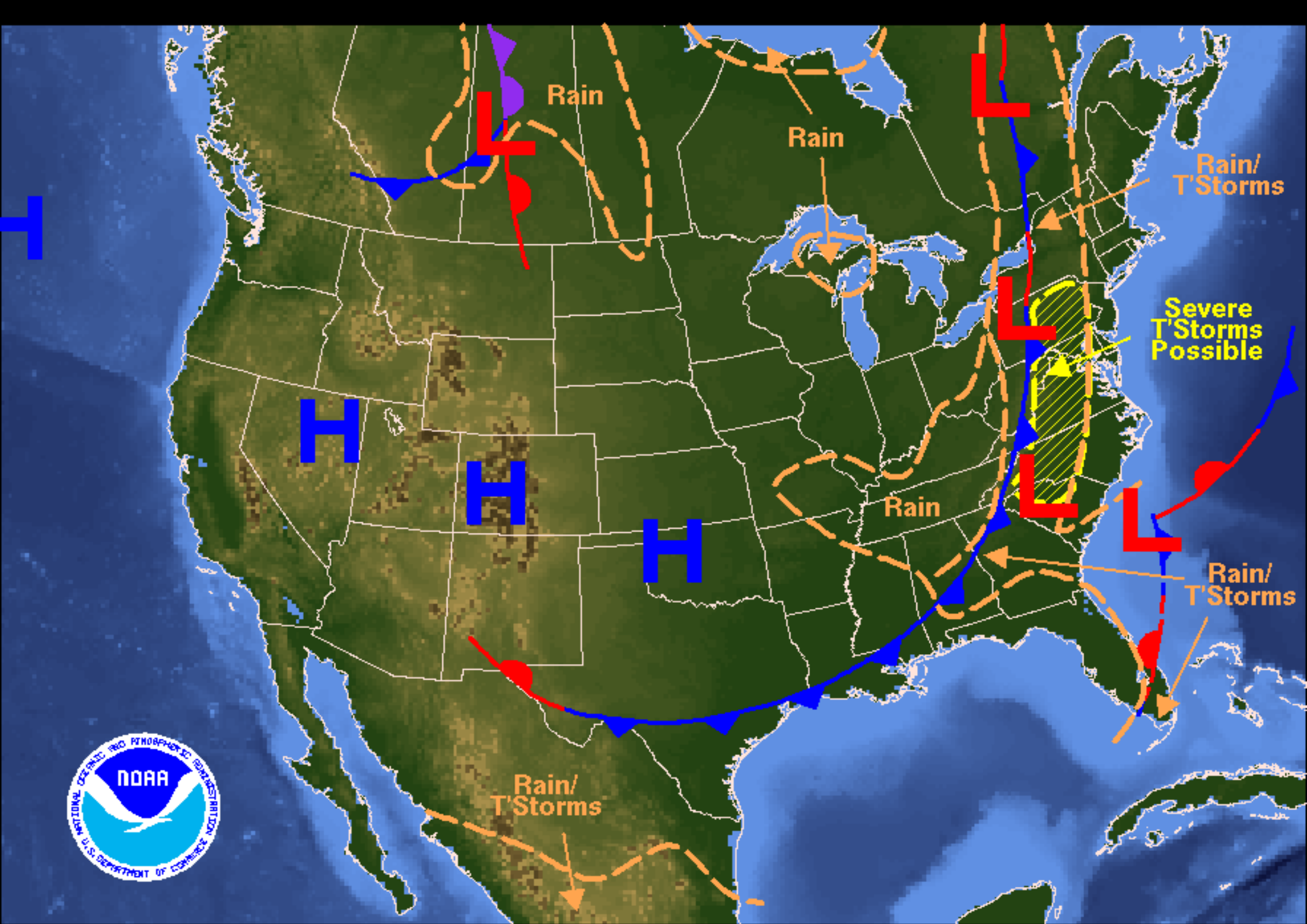
Weather Forecast for Thursday, September 28, 2006 DOC/NOAA/NWS/NCEP/Hydrometeorological Prediction Center Prepared by Fracasso based on HPC, SPC, and TPC forecasts.
