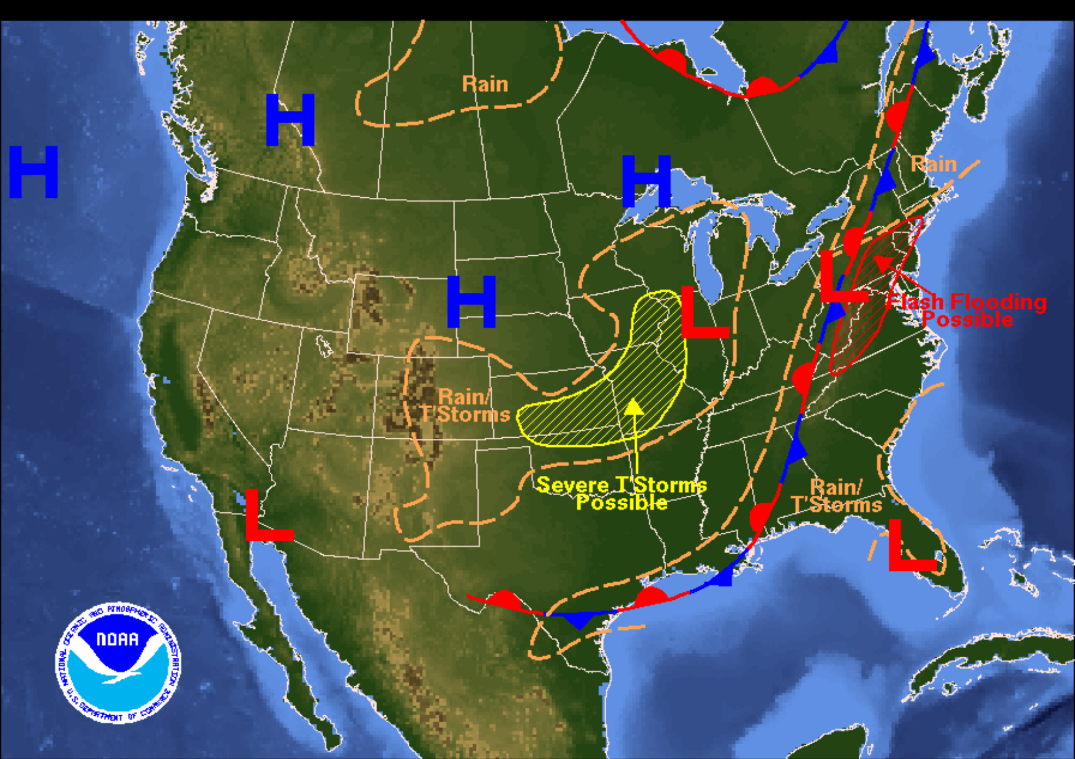
Weather Forecast for Sunday, June 25, 2006 DOC/NOAA/NWS/NCEP/Hydrometeorological Prediction Center Prepared by Fries based on HPC, SPC, and TPC forecasts.
