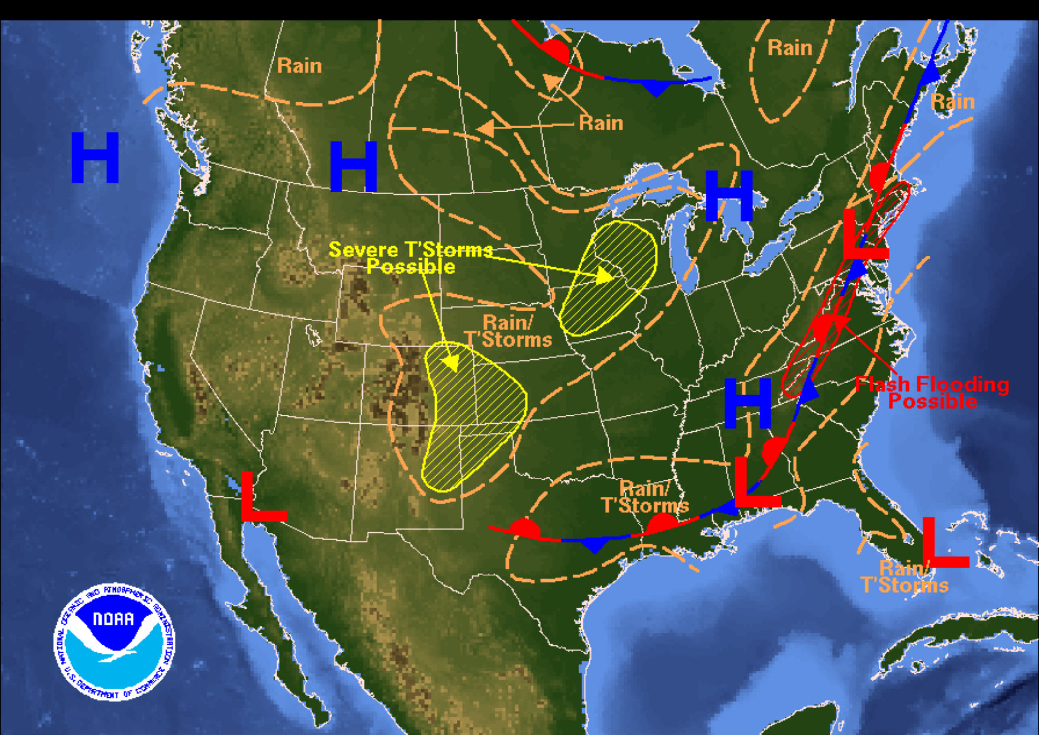
Weather Forecast for Saturday, June 24, 2006 DOC/NOAA/NWS/NCEP/Hydrometeorological Prediction Center Prepared by Fries based on HPC, SPC, and TPC forecasts.
