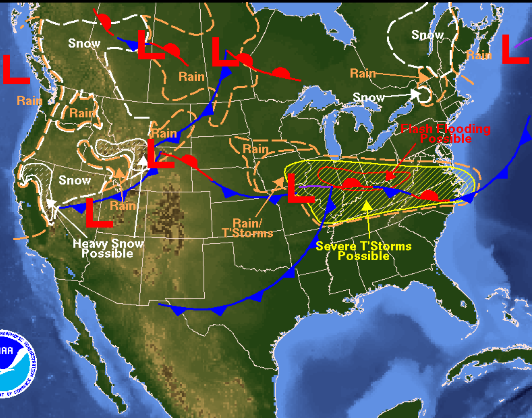
Weather Forecast for Sunday, April 16, 2006 DOC/NOAA/NWS/NCEP/Hydrometeorological Prediction Center Prepared by Fries based on HPC, SPC, and TPC forecasts.
