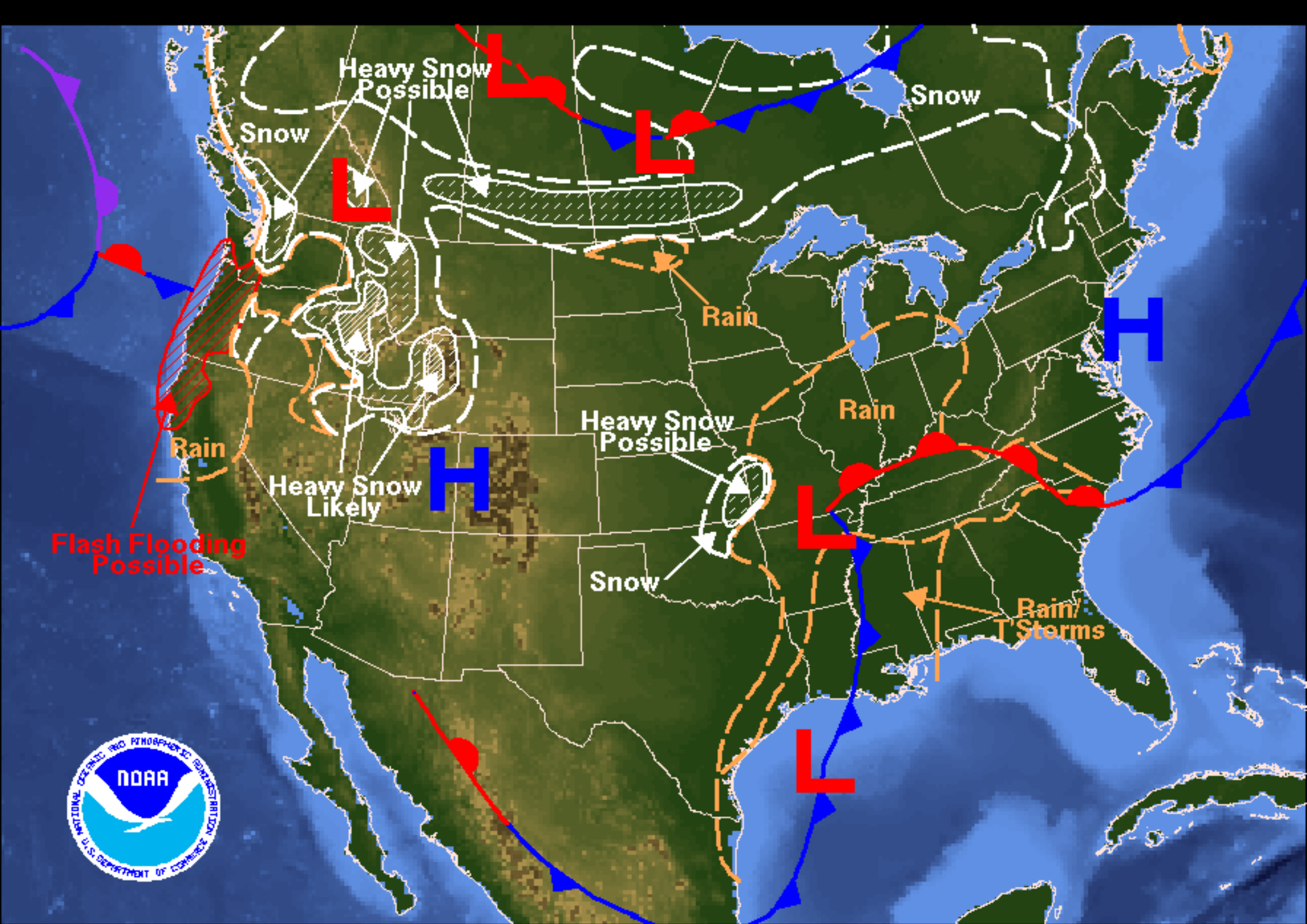
Weather Forecast for Tuesday, January 10, 2006 DOC/NOAA/NWS/NCEP/Hydrometeorological Prediction Center Prepared by Fries based on HPC, SPC, and TPC forecasts.
