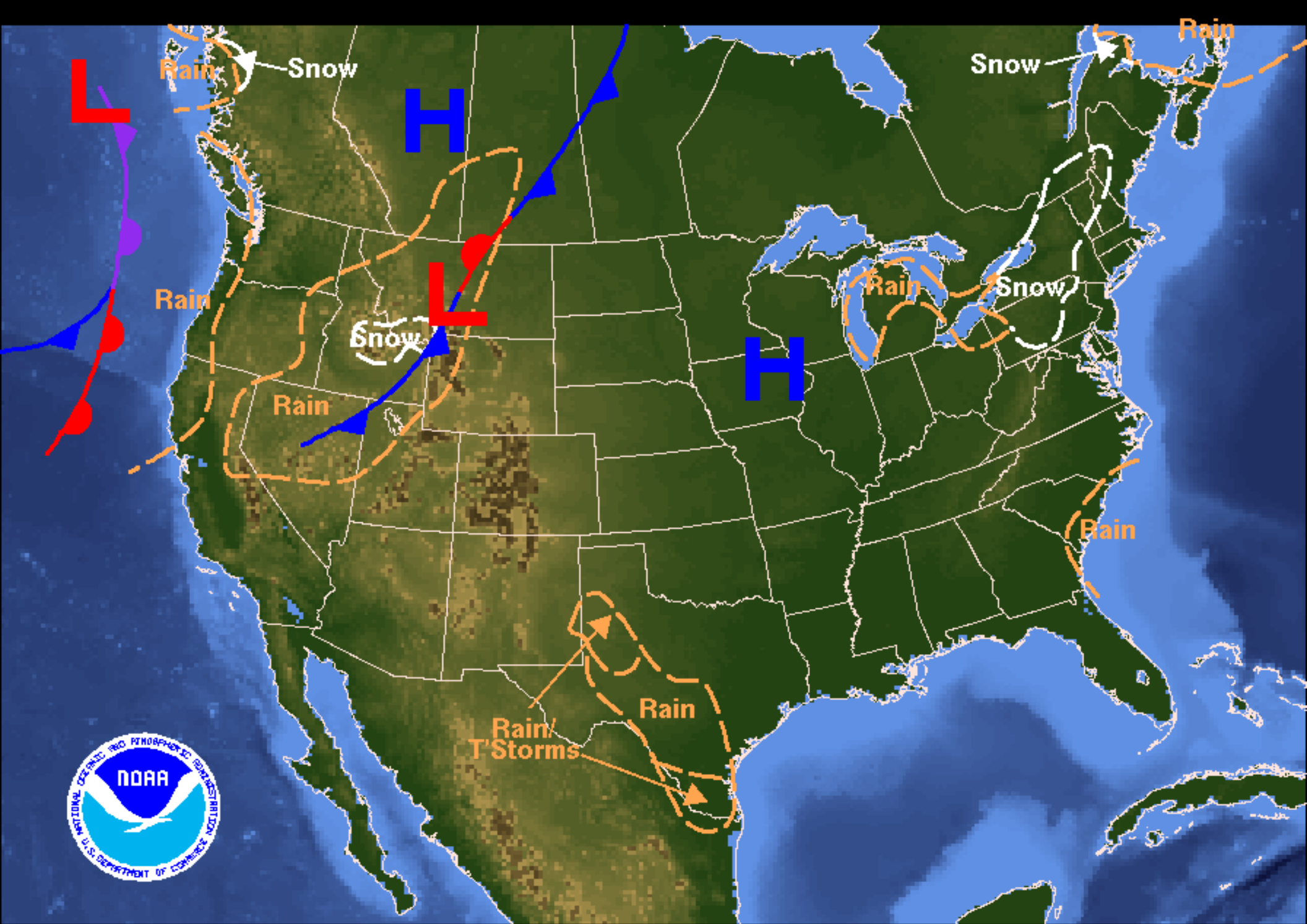
Weather Forecast for Thursday, October 27, 2005 DOC/NOAA/NWS/NCEP/Hydrometeorological Prediction Center Prepared by Trimarco/Terry based on HPC, SPC, and TPC forecasts.
