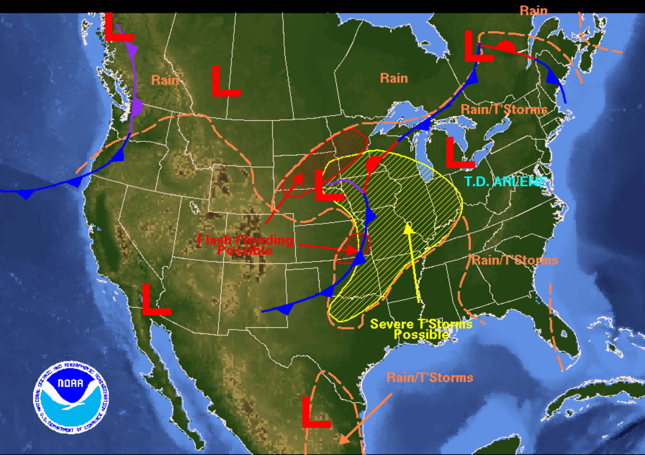
Weather Forecast for Monday, June 13, 2005 DOC/NOAA/NWS/NCEP/Hydrometeorological Prediction Center Prepared by Bell/Terry based on HPC, SPC, and TPC forecasts.
