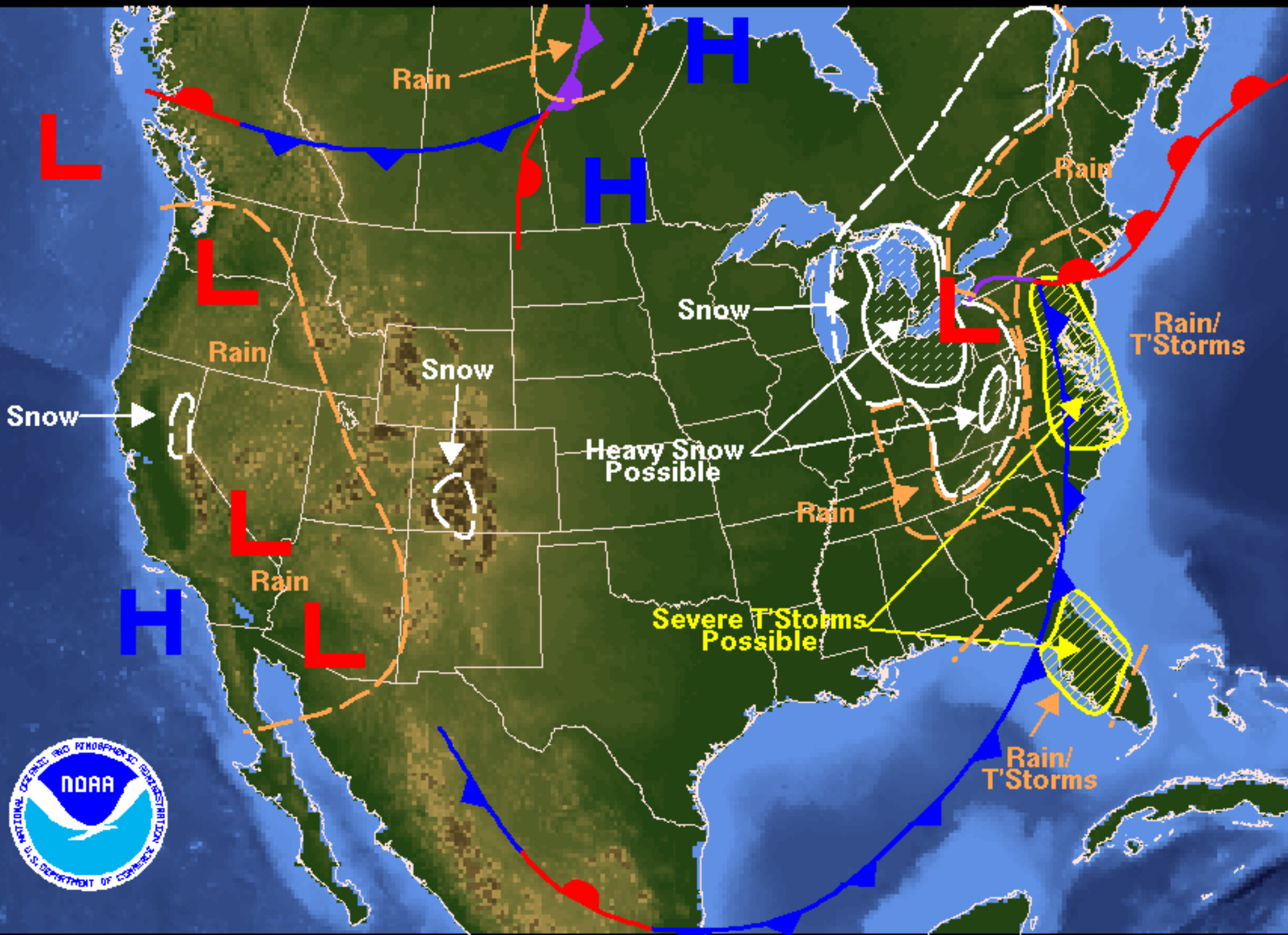
Weather Forecast for Saturday, April 23, 2005 DOC/NOAA/NWS/NCEP/Hydro-meteorological Prediction Center Prepared by SzataneK/Oravec based on HPC, SPC, and TPC forecasts.
