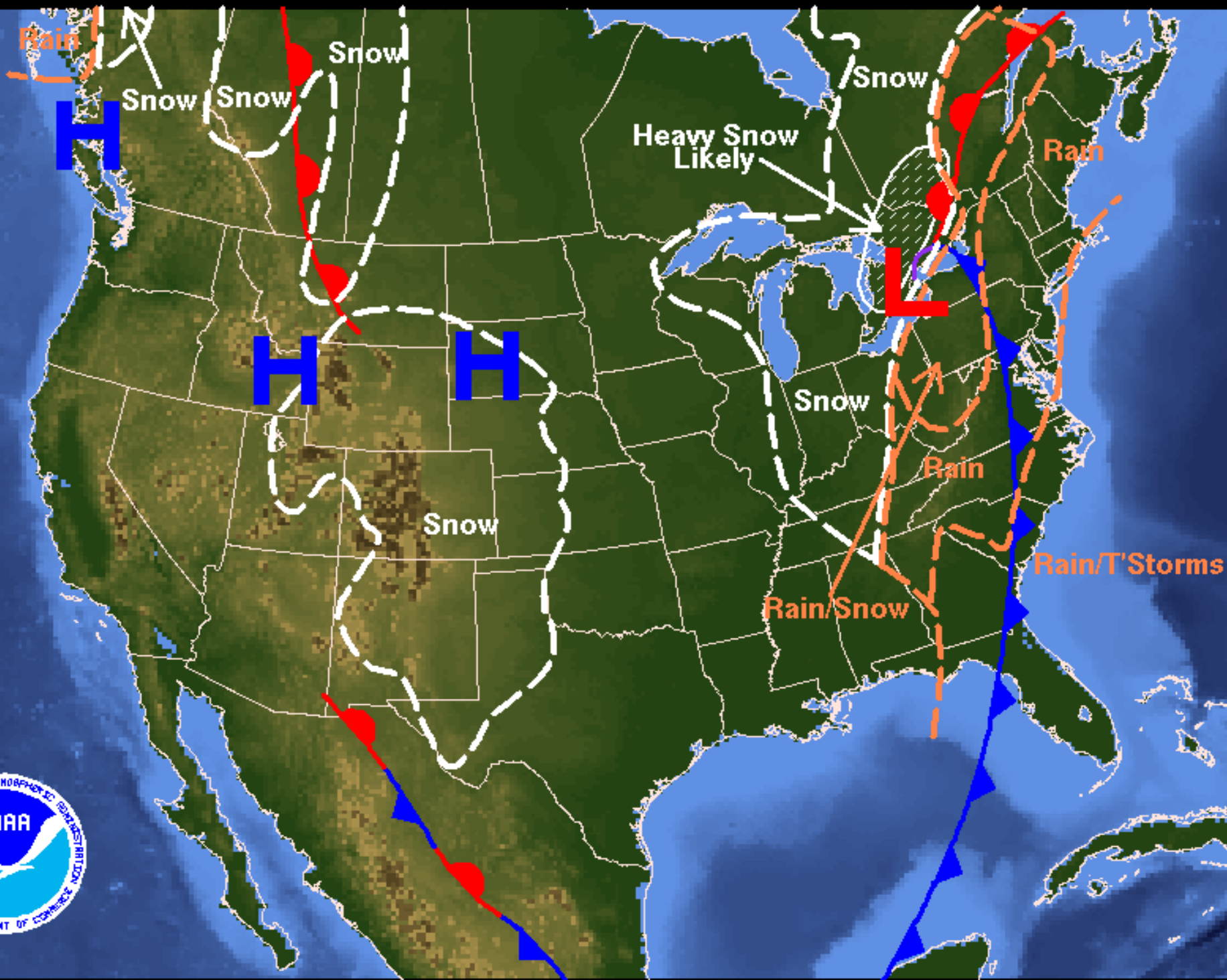
Weather Forecast for Thursday, December 23, 2004 DOC/NOAA/NWS/NCEP/Hydrometeorological Prediction Center Prepared by Halbach/Korty based on HPC, SPC, and TPC forecasts.
