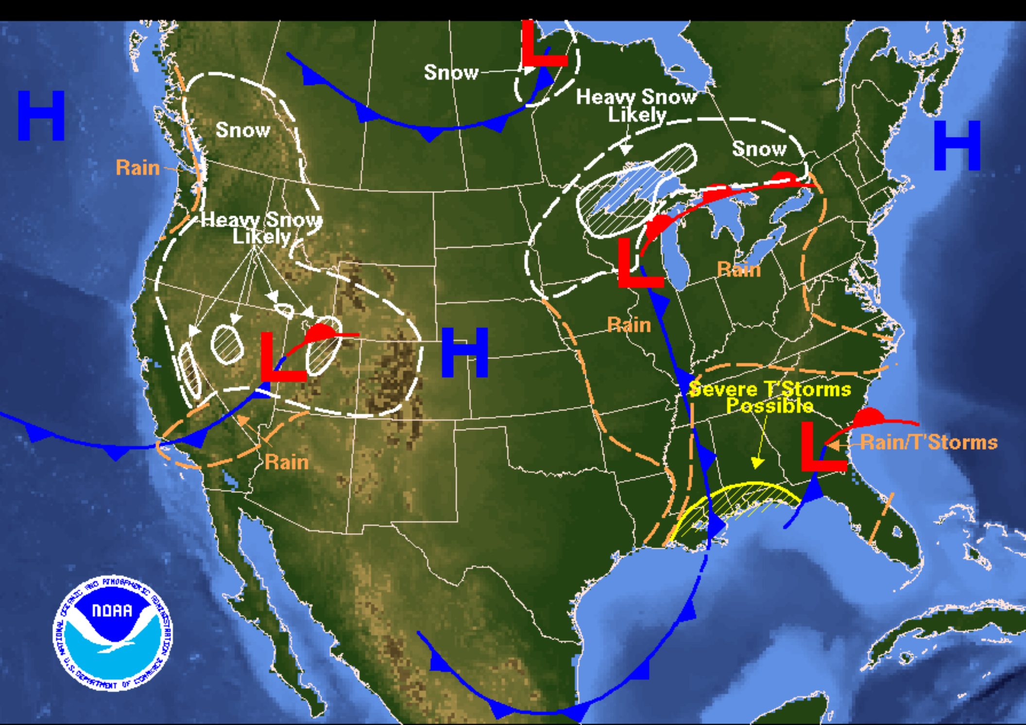
Weather Forecast for Saturday, November 27, 2004 DOC/NOAA/NWS/NCEP/Hydrometeorological Prediction Center Prepared by Szatanek/Sullivan based on HPC, SPC, and TPC forecasts.
