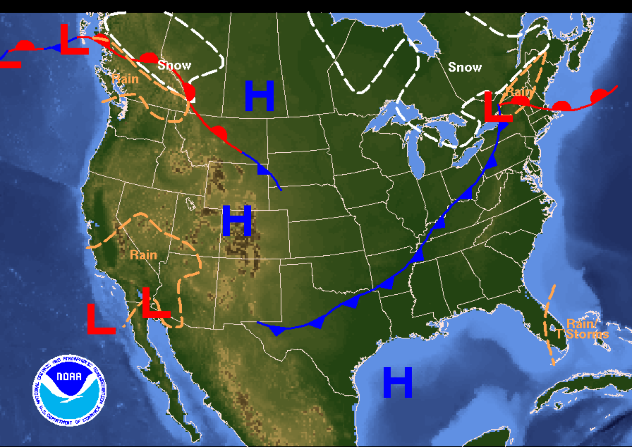
Weather Forecast for Sunday, November 07, 2004 DOC/NOAA/NWS/NCEP/Hydrometeorological Prediction Center Prepared by Lader/Eckert based on HPC, SPC, and TPC forecasts.
