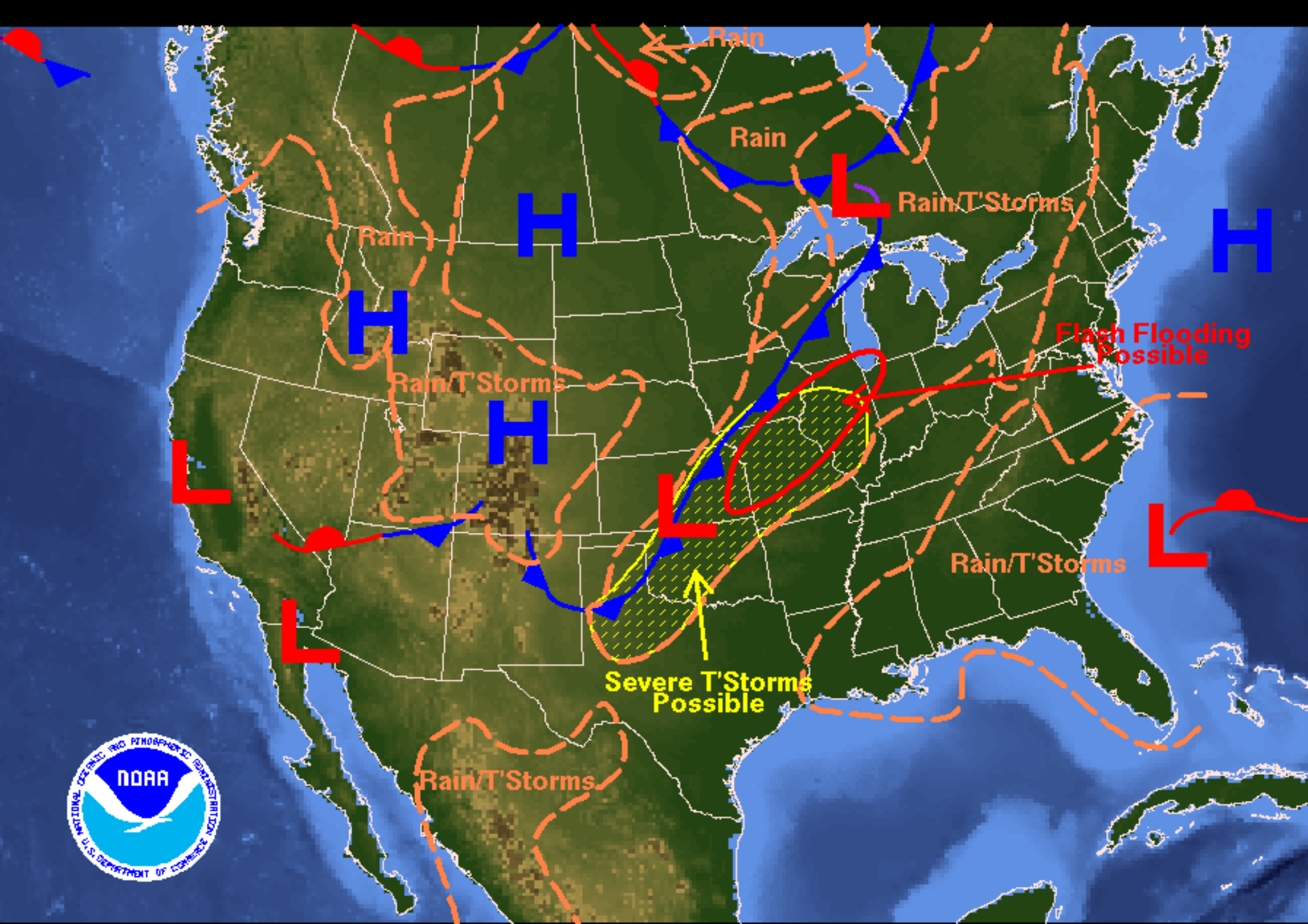
Weather Forecast for Friday, August 27, 2004 DOC/NOAA/NWS/NCEP/Hydrometeorological Prediction Center Prepared by Halbach/Eckert based on HPC, SPC, and TPC forecasts.
