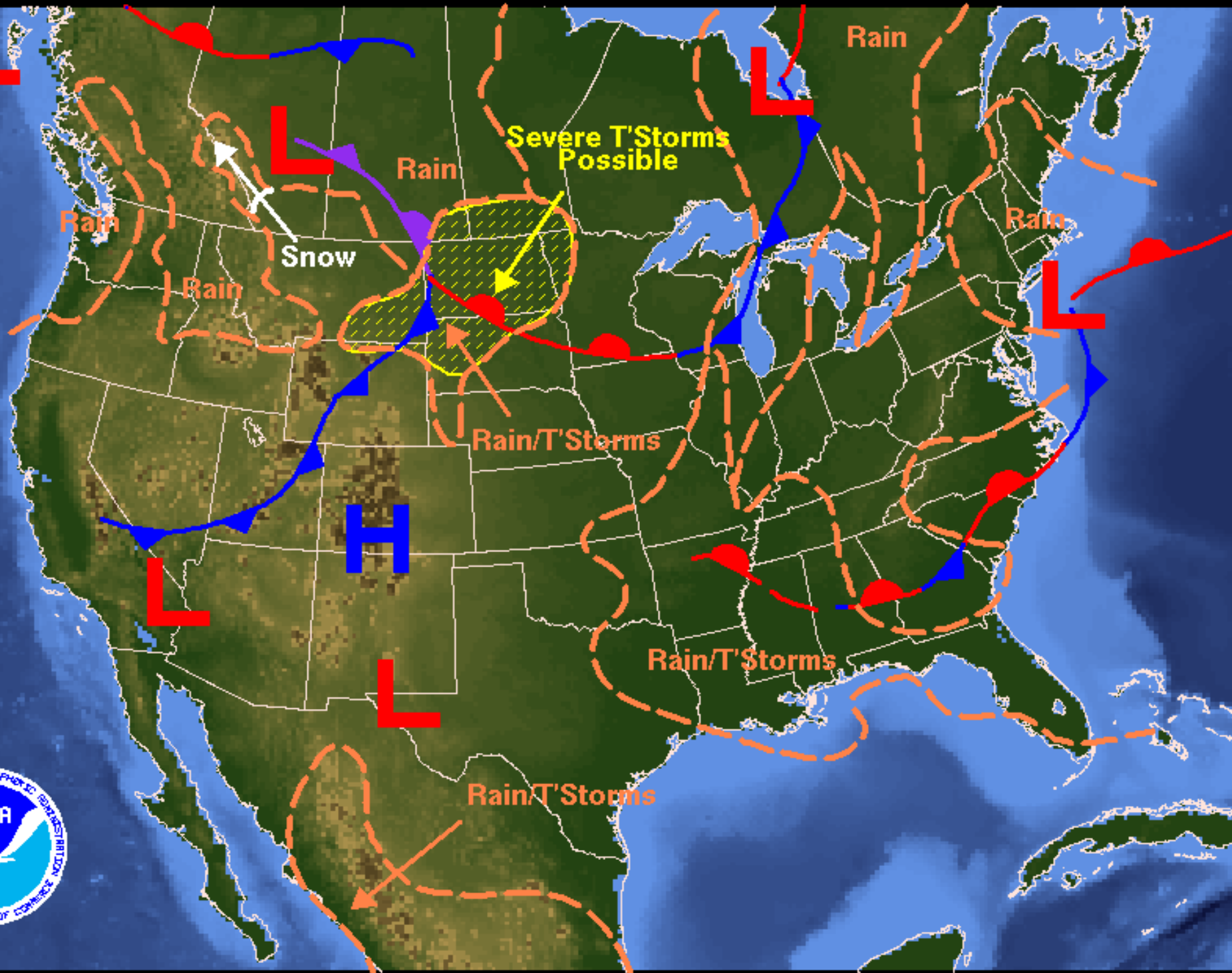
Weather Forecast for Sunday, June 06, 2004 DOC/NOAA/NWS/NCEP/Hydrometeorological Prediction Center Prepared by Bell/Sullivan based on HPC, SPC, and TPC forecasts.
