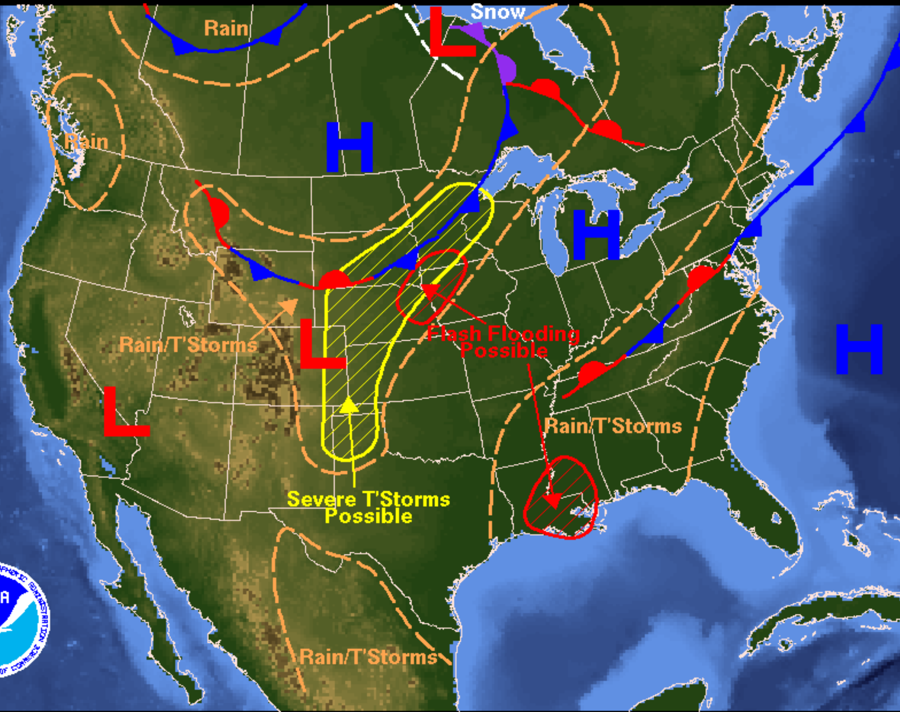
Weather Forecast for Sunday, May 16, 2004 DOC/NOAA/NWS/NCEP/Hydrometeorological Prediction Center Prepared by Szataneck/Eckert based on HPC, SPC, and TPC forecasts.
