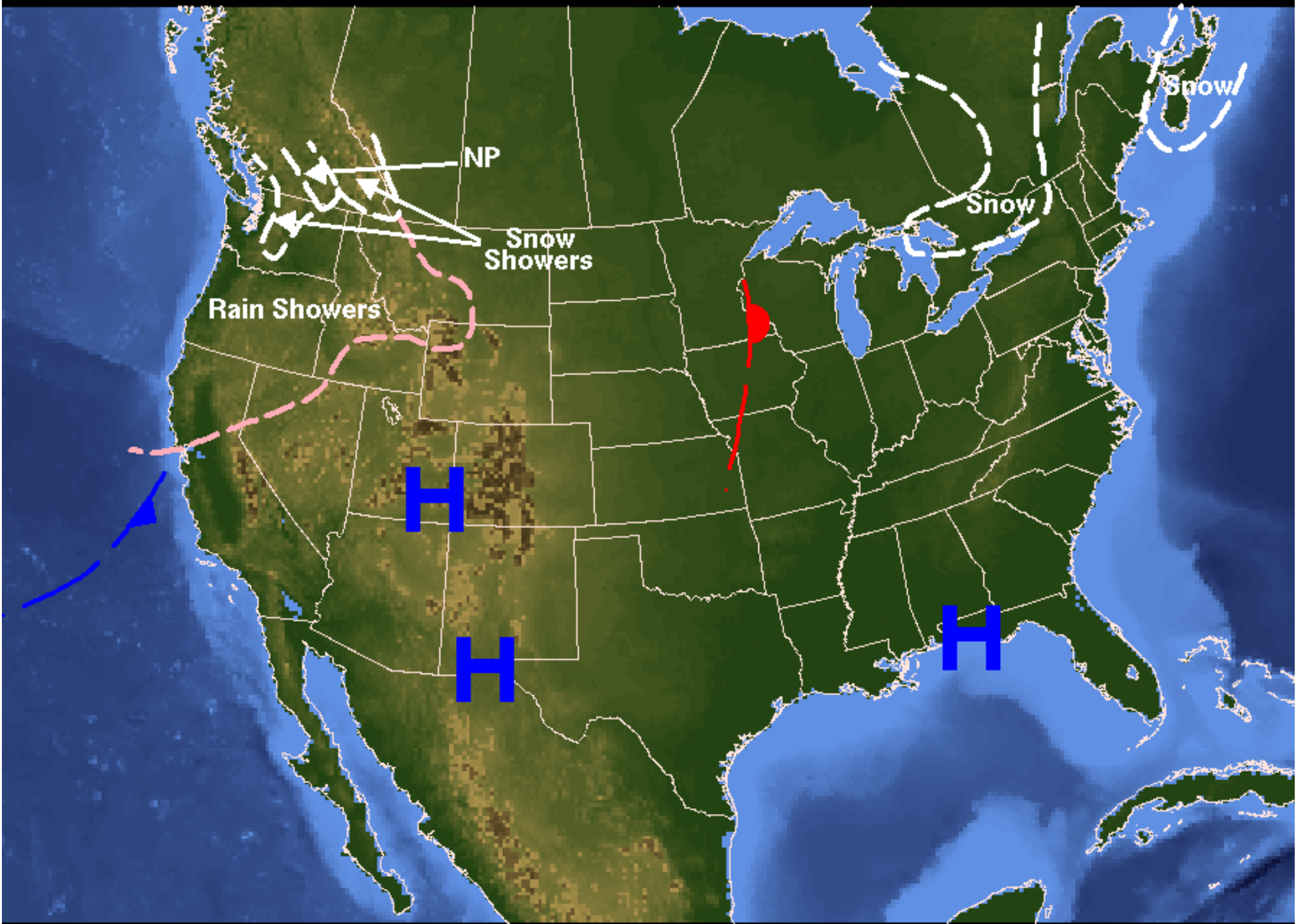
Weather Forecast for Tuesday, January 08, 2002 Prepared by HATCHETT/KORTY
