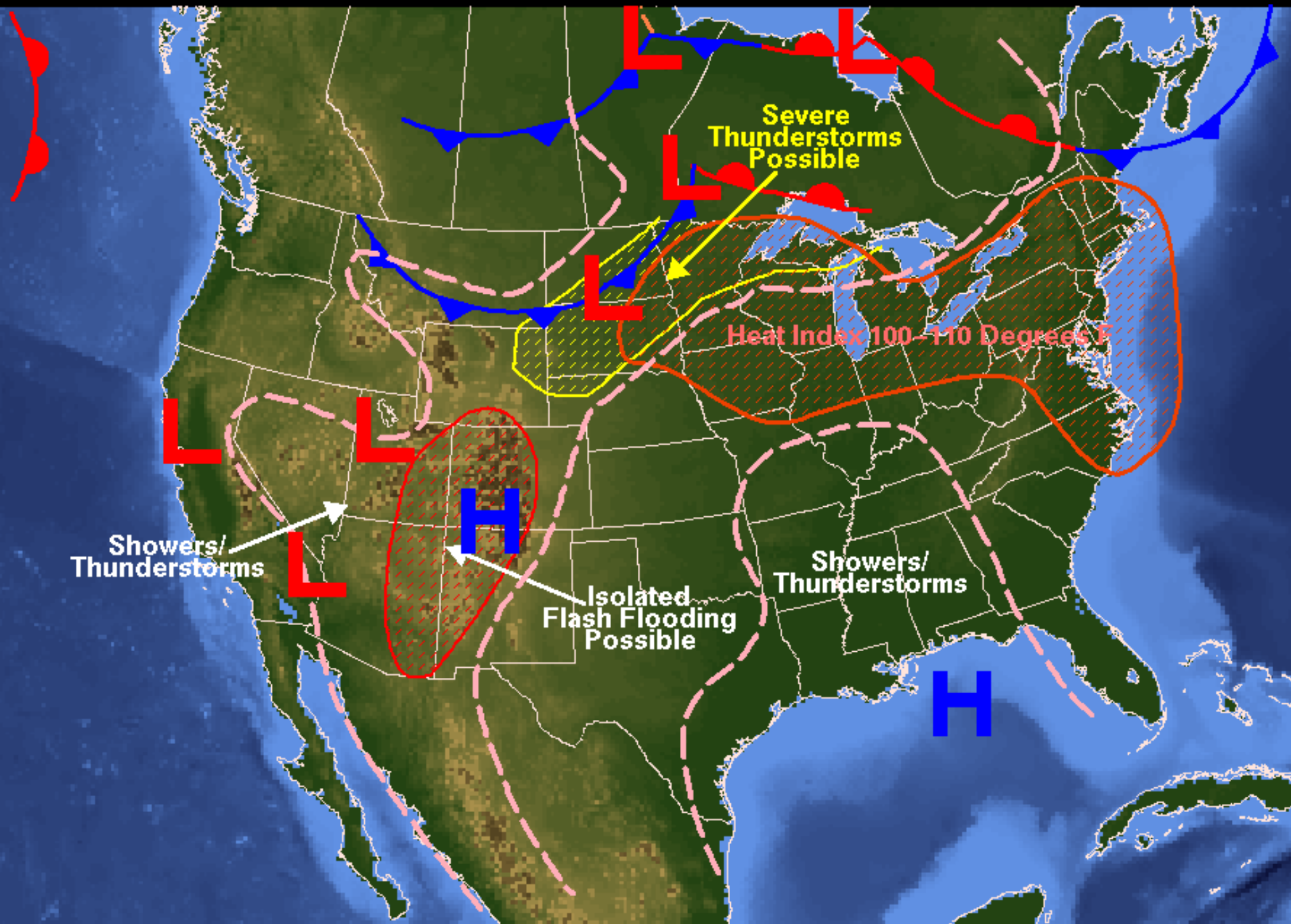
Weather Forecast for Wednesday, August 08, 2001 Prepared by HATCHETT/ECKERT DOC/NOAA/NWS/NCEP/Hydrometeorological Prediction Center
