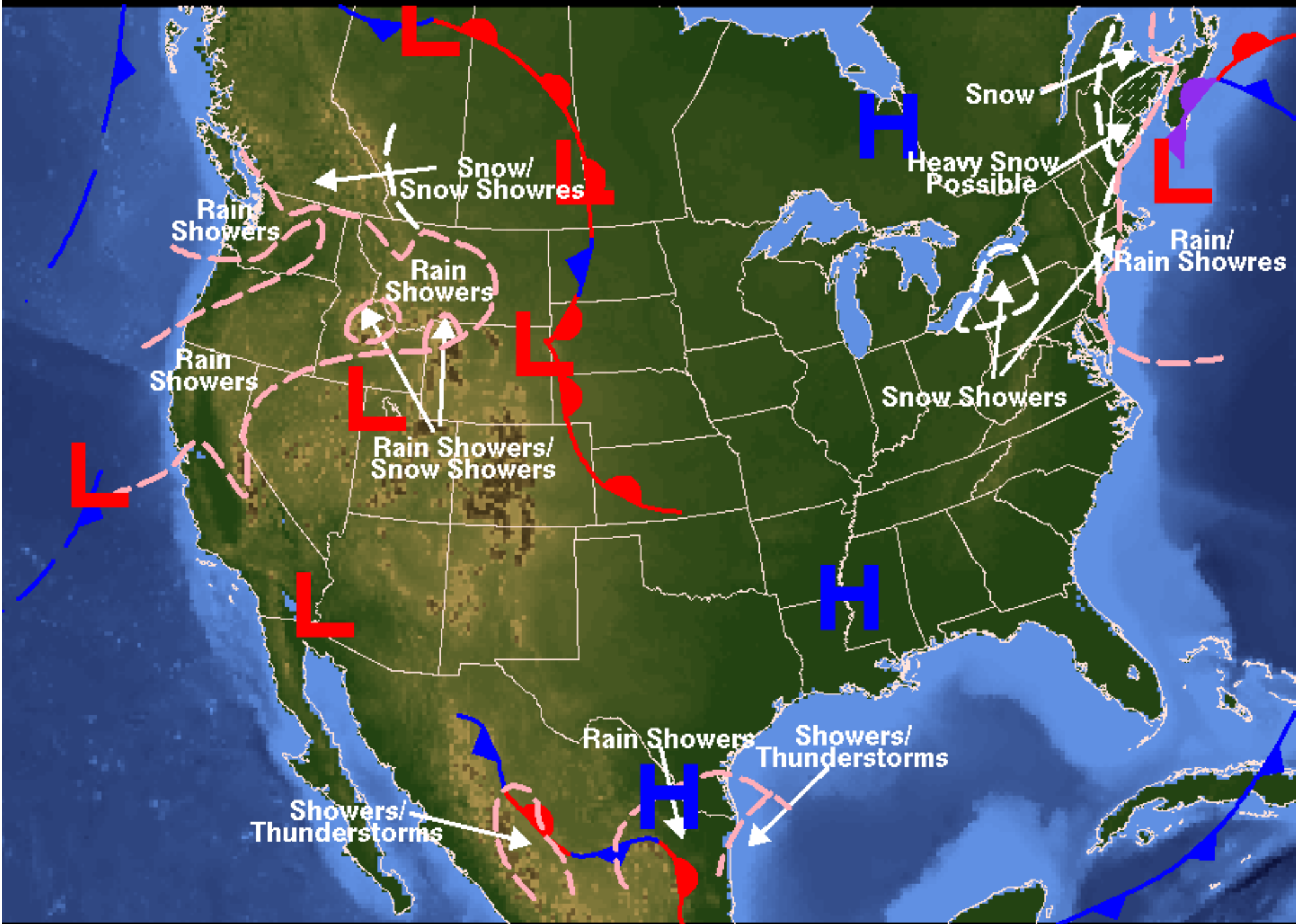
Weather Forecast for Wednesday, April 18, 2001 Prepared by HATCHETT/WOLF DOC/NOAA/NWS/NCEP/Hydrometeorological Prediction Center
