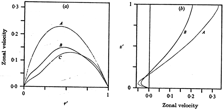
FIGURE 5. Zonal velocity profiles. (a) Vertically averaged profiles of (A) axisymmetric u , (B) wave \bar{u} and (C) scaled-wave angular momentum \frac{1}{2}r\bar{u} . (b) Radially averaged profiles of (A) axisymmetric u and (B) wave \bar{u} , in \text{cm sec}^{-1} .
