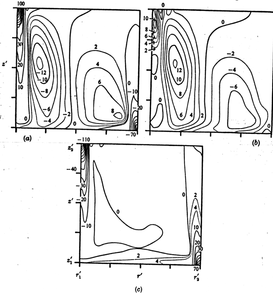
FIGURE 20. Components of the mean temperature equation (27). (a) Mean circulation flux -\langle \bar{v} \bar{T}_r + \bar{w} \bar{T}_z \rangle , (b) deviatoric flux -\langle [(1/r)(r\bar{v}'T')_r + (w'T')_z] \rangle , (c) \kappa \nabla^2 \bar{T} . Units are 10^{-3} \text{ sec}^{-1} .
