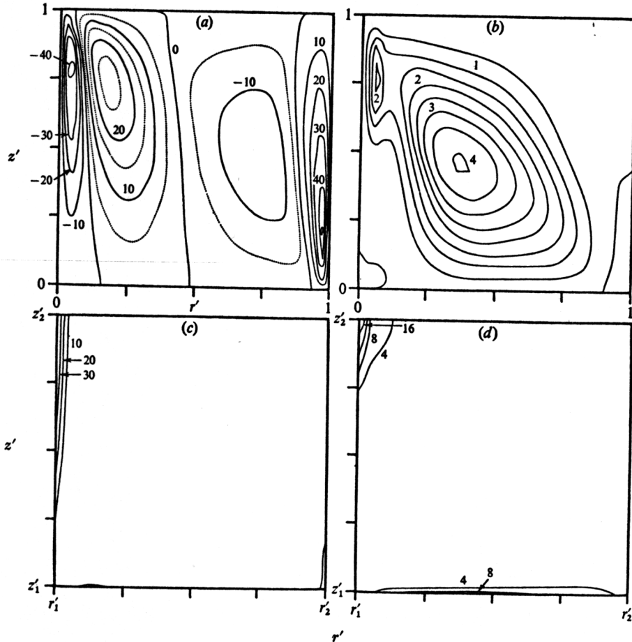
FIGURE 14. Local variation of energy sources and sinks (a) \beta g \bar{w} T' in 10^{-3} \text{ cm}^2 \text{ sec}^{-3} , (b) \beta g w' T' in 10^{-3} \text{ cm}^2 \text{ sec}^{-3} , (c) \bar{\epsilon}^2 in 10^{-3} \text{ cm}^2 \text{ sec}^{-3} , (d) \bar{\epsilon}'^2 in 10^{-3} \text{ cm}^2 \text{ sec}^{-3} from equations (22) and (23). The co-ordinates cover interior ranges r'_1, z'_1 = \frac{1}{64} and r'_2, z'_2 = \frac{9}{64} .
