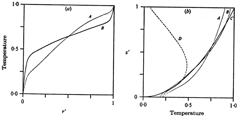
FIGURE 6. Temperature profiles. (a) Vertically averaged profile of \bar{T}/\Delta T for (A) axisymmetric (B) wave mean. (b) Radially averaged profile of \bar{T}/\Delta T for (A) axisymmetric, (B) wave mean, (C) is (z/d)^{1/2} and (D) is the temperature differential across the interior of the fluid, \Delta_I \bar{T}/\Delta T , where \Delta_I \bar{T} = \{\bar{T} \text{ at } r' = \frac{3}{4}\} \text{ minus } \{\bar{T} \text{ at } r' = \frac{1}{4}\} . Mean temperatures are 0.672, 0.670 for axisymmetric and wave solutions.
