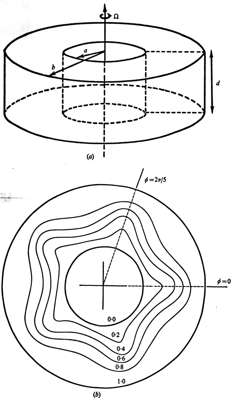
FIGURE 1. (a) Configuration of the system (close to actual size). (b) Pressure wave at upper surface. Container rotates counterclockwise at \Omega = 0.8 \text{ rad sec}^{-1} and the wave rotates counterclockwise relative to the container at \Omega^* = 0.033 \text{ rad sec}^{-1} . Domain of interest is \phi = 0^\circ to 72^\circ . The pressure is normalized in terms of the maximum and minimum values which are 1.8319 and 0.6974 \text{ cm}^2 \text{ sec}^{-2} .
