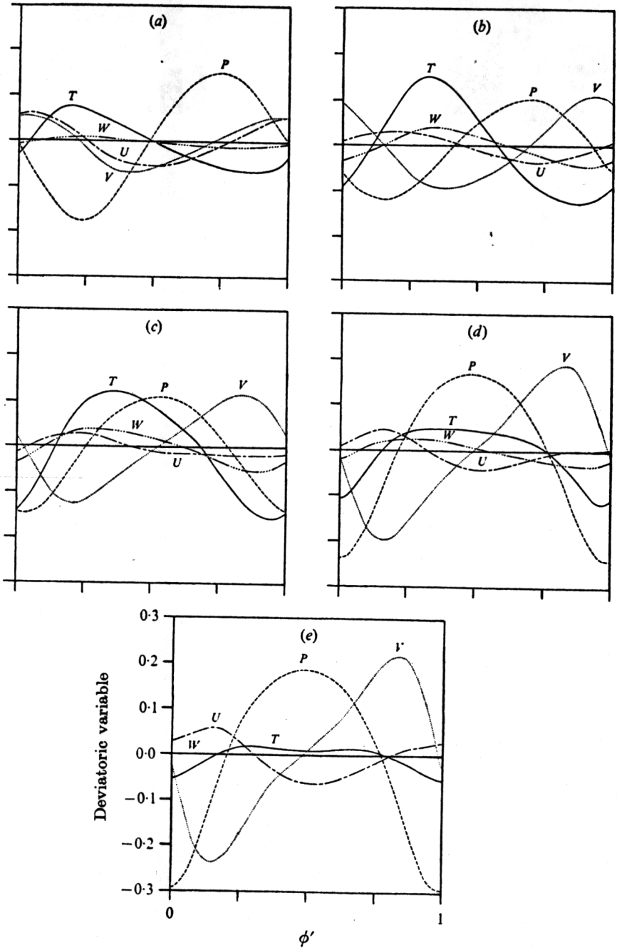
FIGURE 10. Deviatoric wave fields at r' = \frac{1}{2} shown in amplitude versus azimuth form at different heights. The variables are ( P ) \pi' \text{ cm}^2 \text{ sec}^{-2} , ( T ) T'/\Delta T , ( W ) w' \text{ cm sec}^{-1} , ( U ) u' \text{ cm sec}^{-1} and ( V ) v' \text{ cm sec}^{-1} . The heights are z' = : (a) \frac{1}{8} , (b) \frac{1}{4} , (c) \frac{3}{8} , (d) \frac{5}{8} , (e) \frac{7}{8} (i.e. approximately \frac{1}{4} intervals). Co-ordinates all as in (e).
