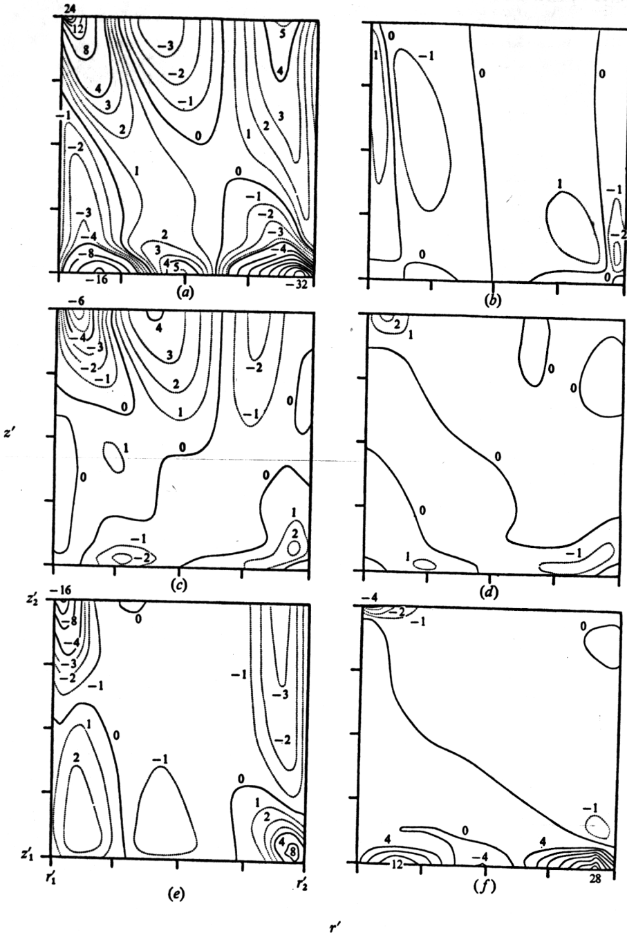
FIGURE 18. Components of the mean angular momentum equation (24). (a) -\bar{v}m_r , (b) -\bar{w}m_z , (c) -1/r(\overline{r v' m'})_r , (d) -(\overline{w' m'})_z , (e) v r (\overline{m_r/r})_r , (f) v \overline{m_{zz}} . The co-ordinates cover the interior grid points of u , i.e. r'_1, z'_1 = \frac{1}{64} ; r'_2, z'_2 = \frac{33}{4} . Units 10^{-2} \text{ cm}^2 \text{ sec}^{-2} . A reduced contouring interval is used for interior regions.
