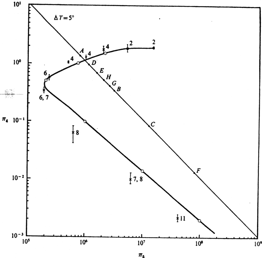
FIGURE 2. Transition curve between axisymmetric motion (to the left) and wave motion constructed from data of Fowles & Hide (1965) for the parameters of the calculation. Co-ordinates are the thermal Rossby \pi_4 and Taylor \pi_5 numbers. Circled values come from the summary curves of Fowles & Hide interpreted for our parameter values. Cross marks indicate transition points for observations with small fluid depth (5 cm) and square marks are likewise for small inner radius. Associated wave-numbers are given as a guide. The diagonal line \Delta T = 5^\circ \text{ C} is locus of interest. The solution is obtained at H ( \Omega = 0.8 ). Other points on the line have values of \Omega , A = 0.5, D = 0.6, E = 0.7, H = 0.8, G = 0.9, B = 1.0, C = 2.0, F = 5.0. The symmetric to wave transition occurs near \Omega = 0.55 and irregular flow occurs near point C .
