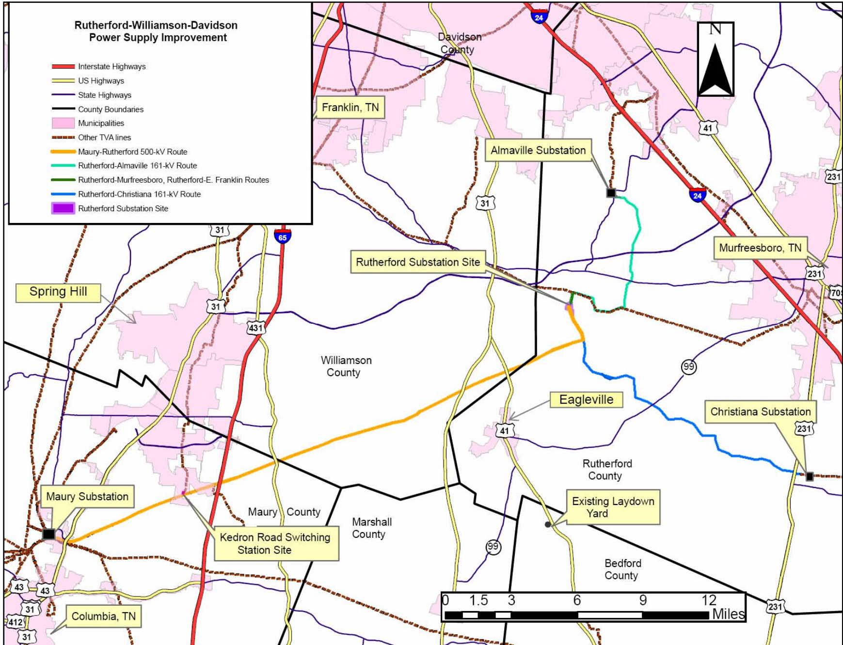
Figure S-1. Proposed Rutherford 500-kV Substation and Associated 500-kV and 161-kV Transmission Lines
