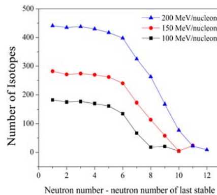
Figure 3: The number of neutron-rich isotopes produced above 0.01 pps as a function of the distance from stability.
