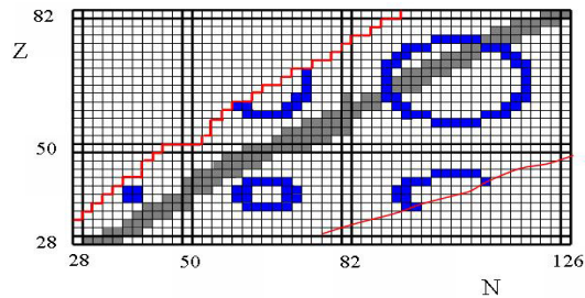
Figure 5: The evolution of collective motion in complex nuclei: many heavier nuclei are expected to exhibit novel collective properties such as (see blue squares) phase transitions in the equilibrium shape.
