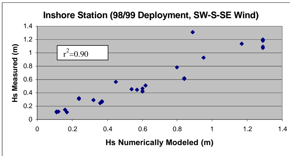
Figure 7.10. Scatter plot of measured and modeled H_s for wind blowing from southwest, south and southeast for 1998/99 deployment at Inshore station.
