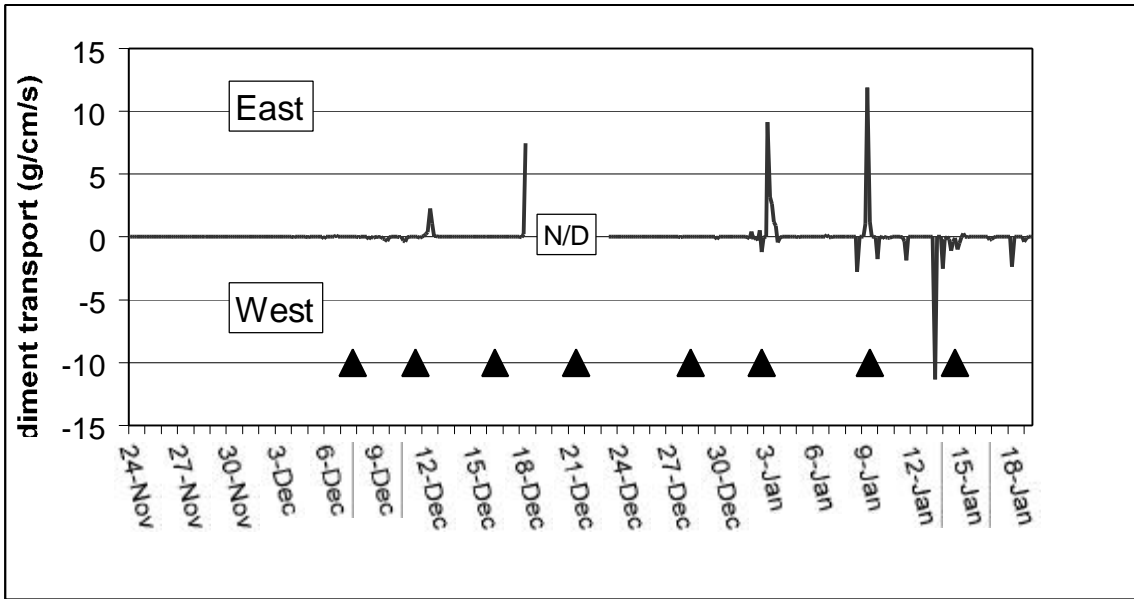
Figure 5.19. Along-shelf longshore sediment transport for Site 1 (System 1A) as predicted using the GMR method.
