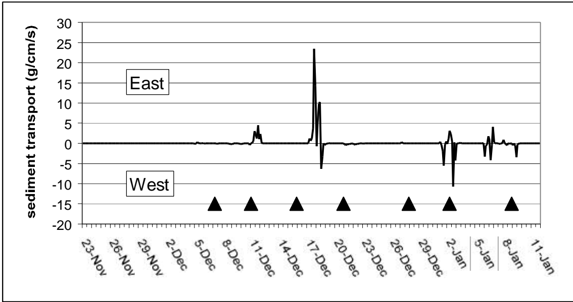
Figure 5.17. Along-shelf cross-shore sediment transport for Site 2 as predicted using the GMR method.
