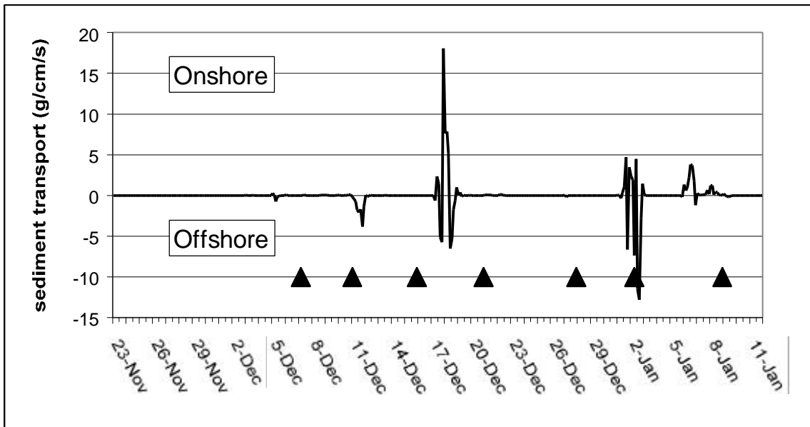
Figure 5.16. Across-shelf longshore sediment transport for Site 2 as predicted using the GMR method.
