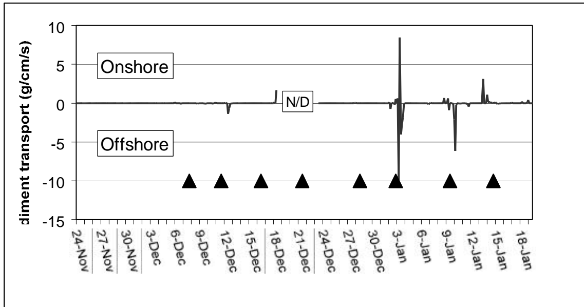
Figure 5.18. Across-shelf cross-shore sediment transport for Site 1 (System 1A) as predicted using the GMR method.
