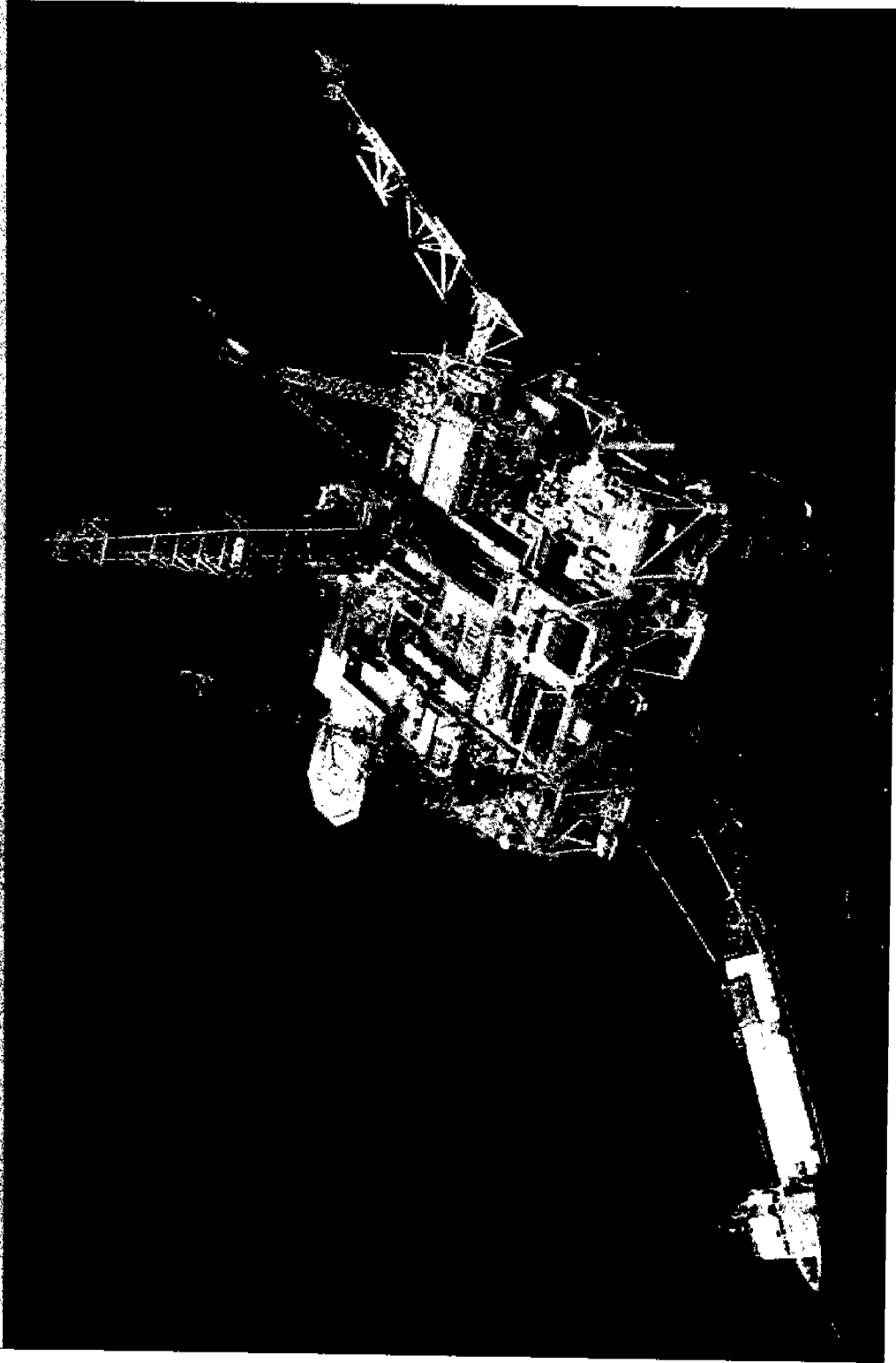
Figure 1J.13. Mars on location.
