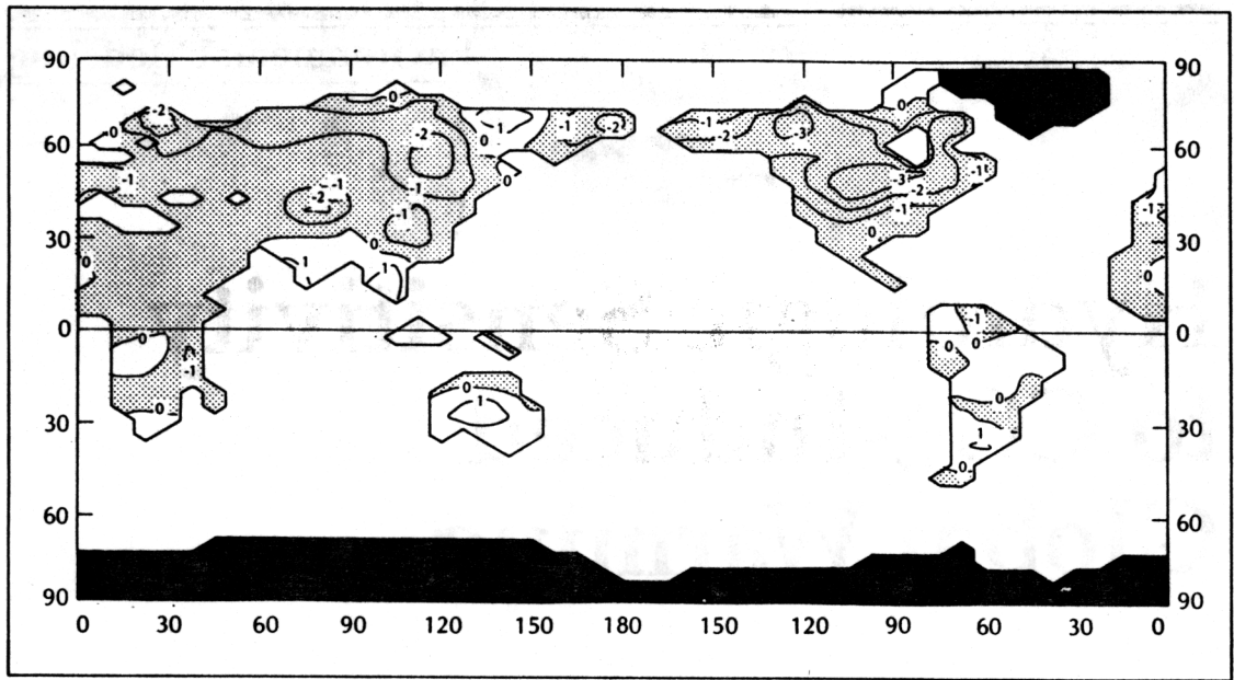
FIGURE 1. The geographical distribution of the difference in soil moisture (cm) between high- \text{CO}_2 and normal- \text{CO}_2 experiments for the June-July-August period.
