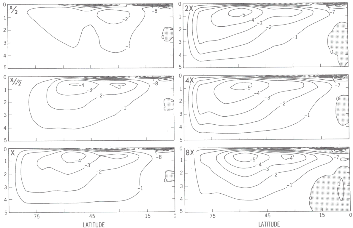
Fig. 13. Streamlines illustrating the meridional circulation in the model ocean from the six experiments. Units are in sverdrups ( 10^{12} g/s). Note that the meridional mass transport illustrated here represents the transport in one (rather than three) ocean sector.
