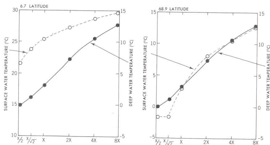
Fig. 12. Zonal mean temperature (in degrees Celsius) of surface water and deep water (depth of 4566 m) at 6.7° latitude (left) and 68.9° latitude (right) of the model ocean from the six experiments.
