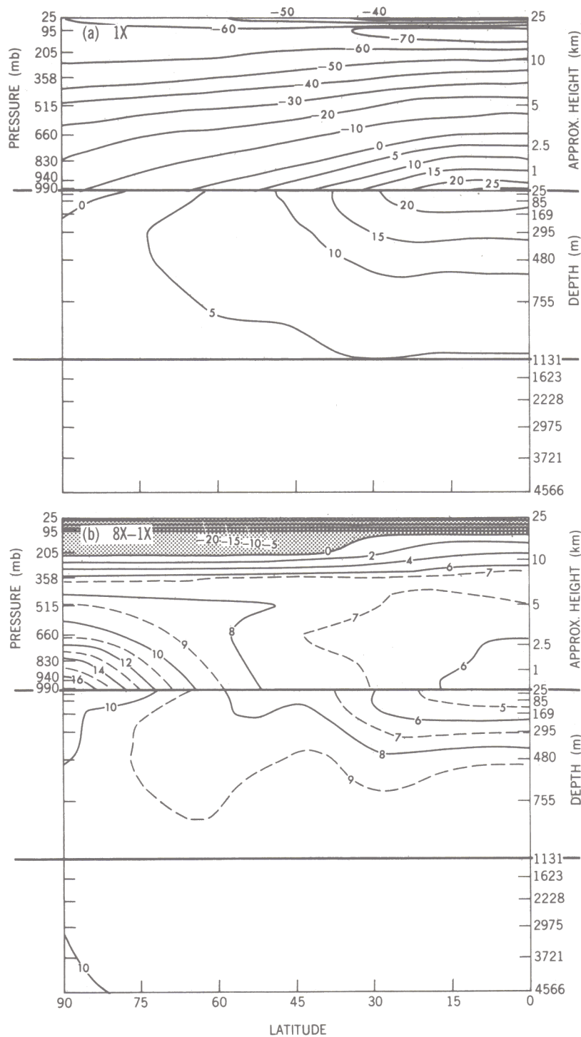
Fig. 3. (a) Zonal mean temperature (in degrees Celsius) of the ocean-atmosphere model from the 1X experiment. (b) The difference in zonal mean temperature (in degrees Celsius) of the ocean-atmosphere model between the 1X and 8X experiments.
