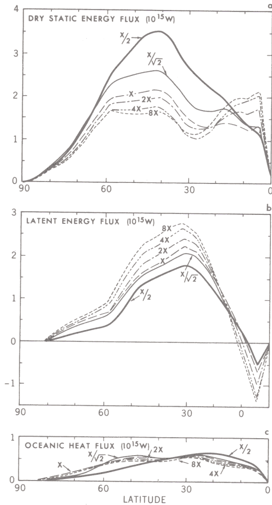
Fig. 16. Poleward transport of (a) dry static energy, (b) latent energy in the model atmosphere, and (c) oceanic heat transport in the six experiments. Units are in 10^{15} W. Note that three sector oceans and three sector atmospheres, which cover an entire hemisphere, are involved in these transports.
