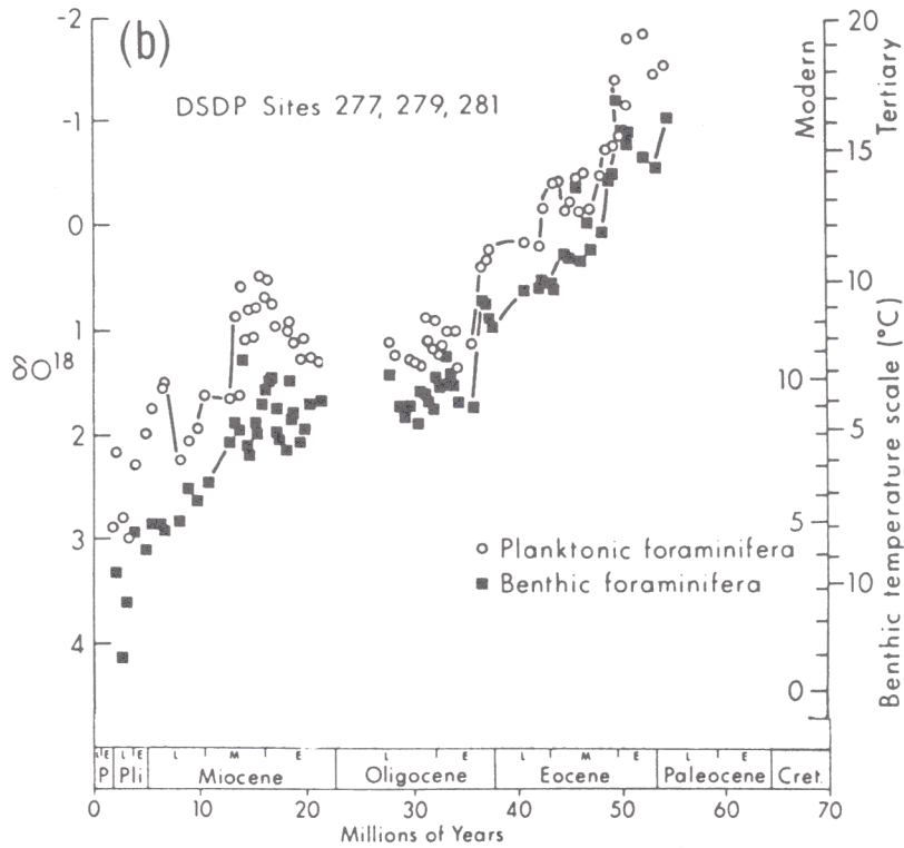
Fig. 11. Isotopic temperature data for Tertiary planktonic foraminifera (open symbols) and benthic foraminifera (solid symbols) compiled by Savin [1977]. The modern and Tertiary benthic temperature scales were calculated assuming water \delta^{18}\text{O} values of -0.08 and -1.00\text{‰} , respectively. (a) Data primarily from the North Pacific sites which are believed to have occupied tropical positions throughout the Late Cretaceous and Tertiary. To estimate isotopic temperatures of planktonic foraminifera, add approximately 2.5^\circ\text{C} to the appropriate benthic temperature scale. (b) Data from the Campbell Plateau and the Macquarie Ridge (Subantarctic Pacific) as analyzed by Shackleton and Kennett [1975]. Because of the extreme oceanographic changes in the area during the Tertiary, a separate temperature scale for planktonic foraminifera was not estimated.
