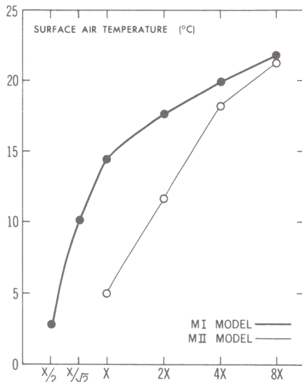
Fig. A2. The area mean surface air temperature from two series of the CO 2 experiments. The thick solid line denotes the MI model. The thin solid line denotes the MII model.
