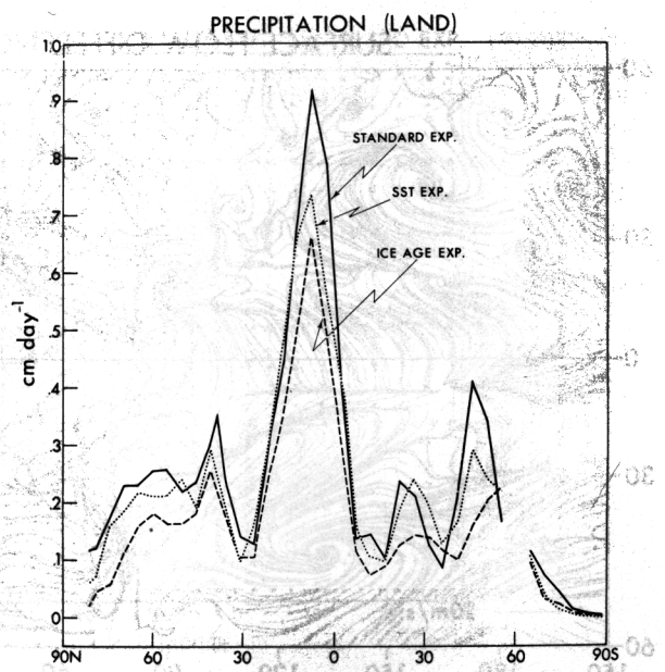
Fig. 24. Latitudinal distributions of zonal mean rate of precipitation (in centimeters per day) over land.
