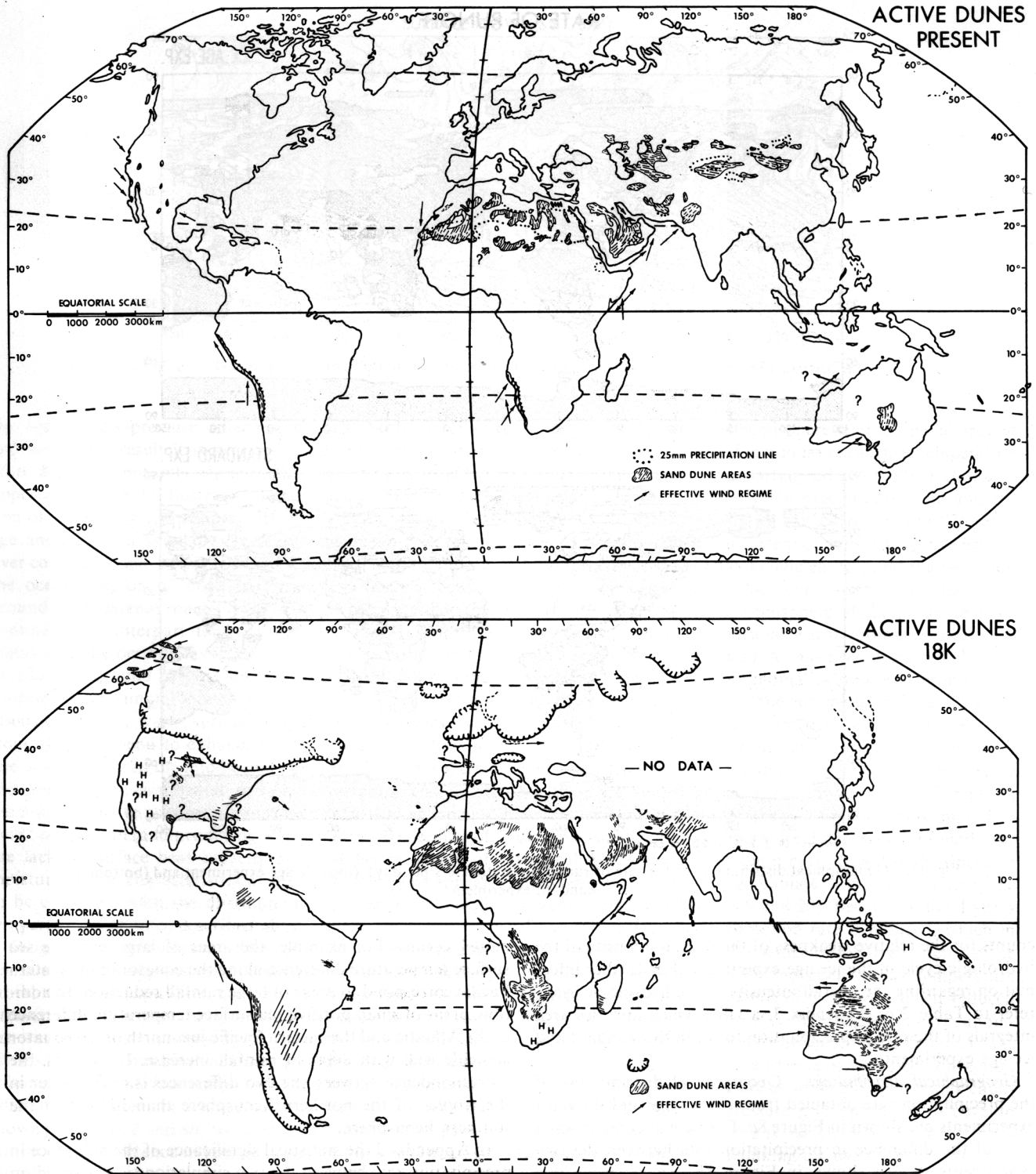
Fig. 10. Geographical distributions of active sand dunes (hand-copied from Sarnthein and Diester-Haass [1977] ): (top) present distribution and (bottom) 18,000 yr B.P. distribution. Spiral lines indicate the margins of glacial ice.
