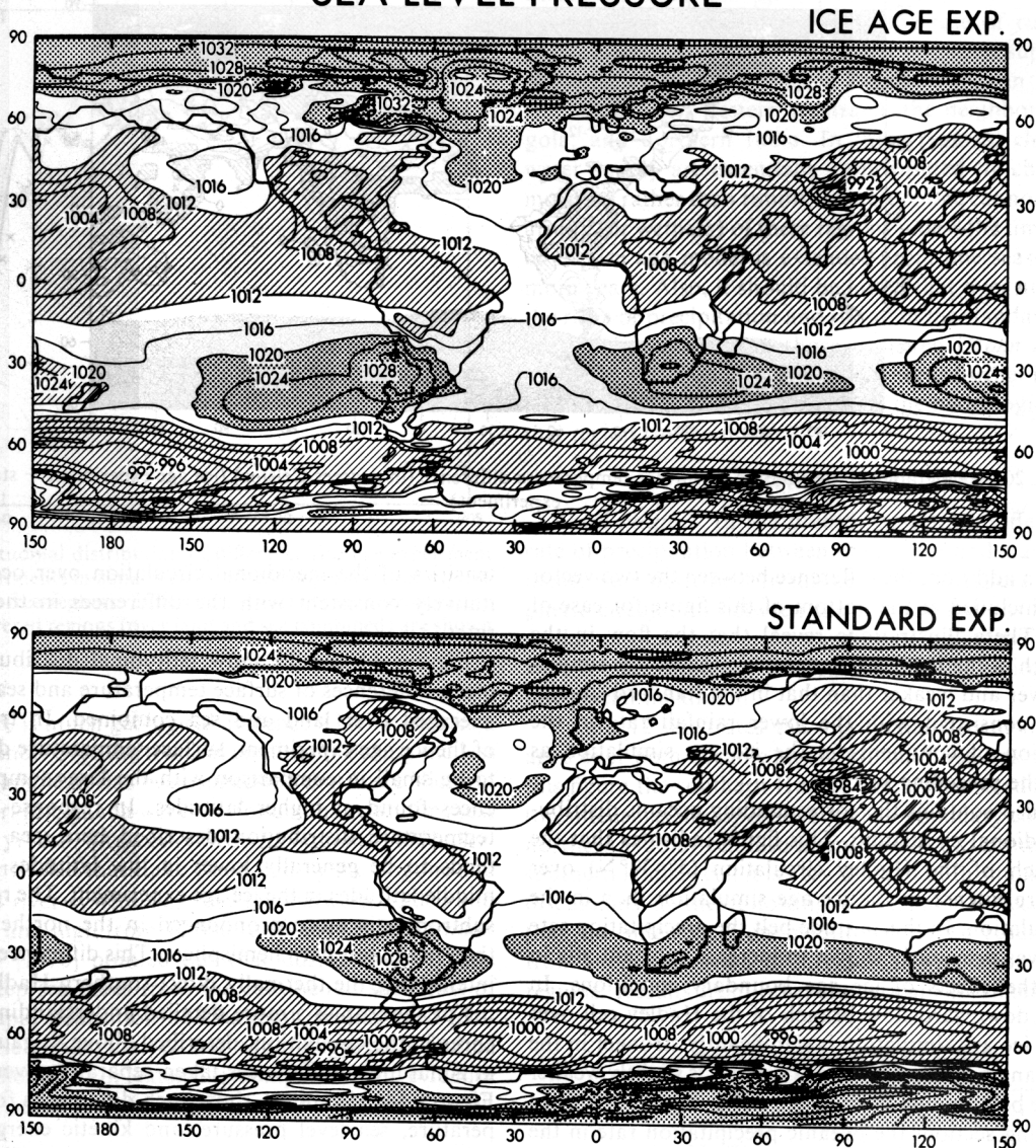
Fig. 19a. Geographical distribution of sea level pressure (in millibars): (top) ice age experiment and (bottom) standard experiment.
