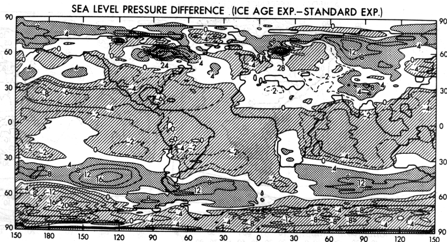
Fig. 19b. Geographical distribution of sea level pressure difference (in millibars) (ice age experiment - standard experiment).
