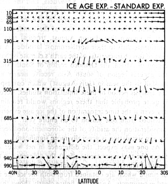
Fig. 13. Zonal mean meridional circulation over land and sea: (top) ice age experiment, (middle) standard experiment, and (bottom) ice age experiment - standard experiment. The length of a vector represents the displacement of an air parcel in 2 days.
