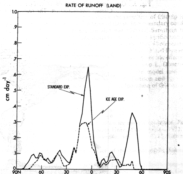
Fig. 7. Latitudinal distributions of zonal mean rate of runoff (in centimeters per day) over continents.
