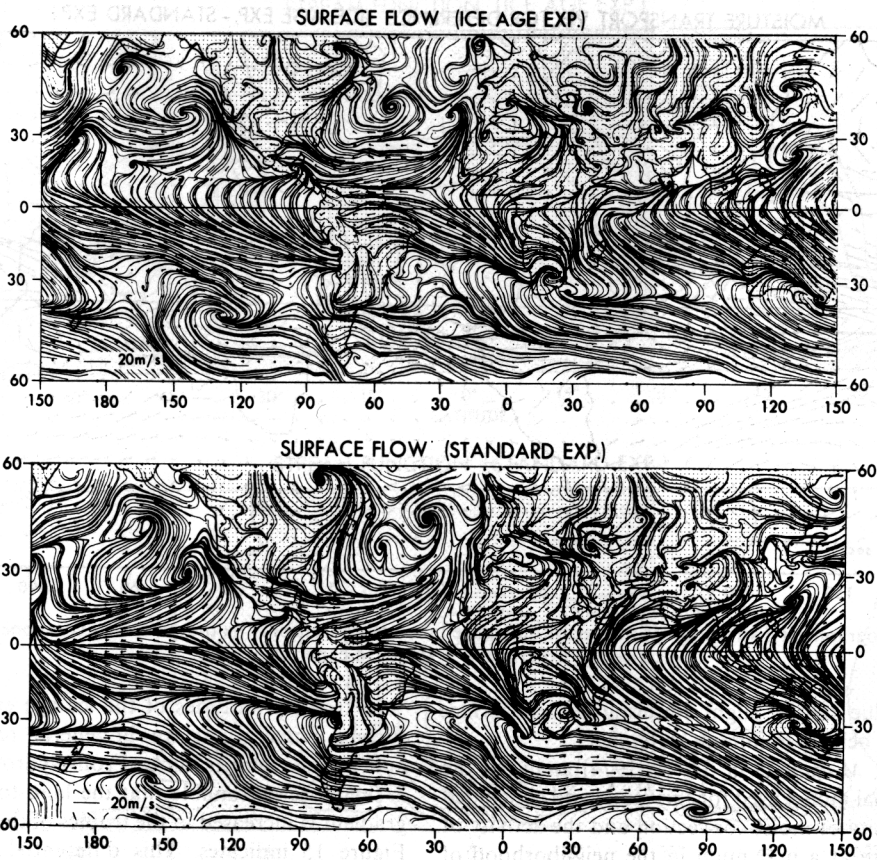
Fig. 22a. Geographical distributions of surface wind vectors: (top) ice age experiment and (bottom) standard experiment.
