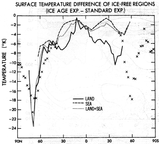
Fig. 14. Latitudinal distribution of difference (ice age experiment standard experiment) in zonal mean surface temperature (in degrees Celsius) over ice-free regions. Differences in zonal mean temperature including ice-covered regions (over land and sea combined) are shown by crosses.
