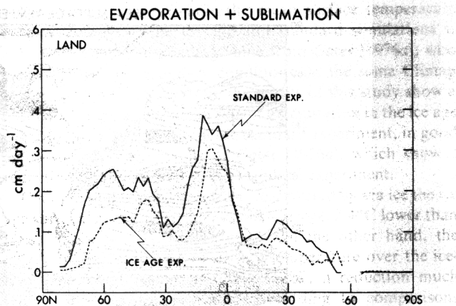
Fig. 6. Latitudinal distributions of zonal mean rate of evaporation + sublimation (in centimeters per day) over continents.
