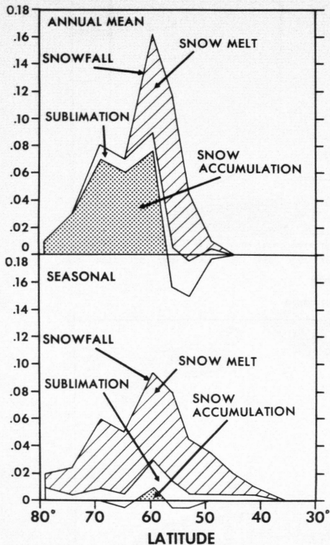
FIGURE 12.—Latitudinal distributions of zonal mean rates of various snow budget components (snowfall, snowmelt, and sublimation) on the continental surface. The rate of snowfall is equal to the sum of the snow budget components shown. Units: cm of water equivalent per day.
