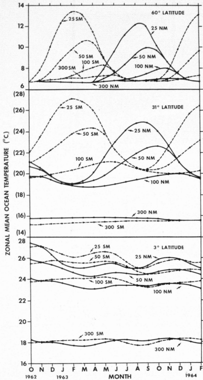
FIGURE 4.—Time variation of zonal mean oceanic temperature ( ^{\circ}\text{C} ) at various depths for both hemispheres at latitudes 60^{\circ} , 31^{\circ} , and 3^{\circ} (from top to bottom), respectively. The entire period of the seasonal integration is shown. The Northern Hemisphere mean values (NM) are represented by solid lines, and the Southern Hemisphere mean values (SM) by dashed lines.
