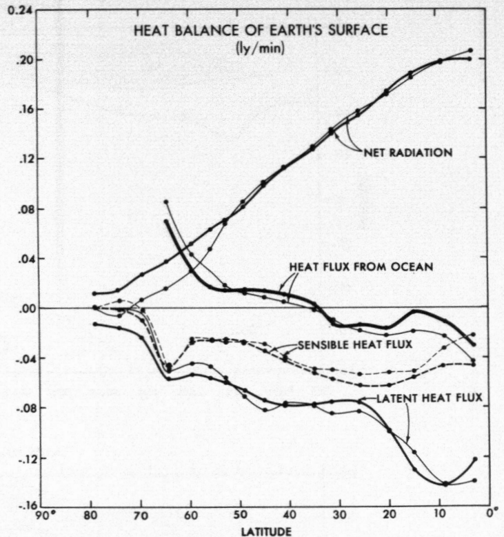
FIGURE 13.—Zonal mean rates of heating (ly/min) of the model surface (both land and sea together), due to net radiation, latent heat flux, sensible heat flux, and heat flow from the interior to the surface of the model ocean. Thick lines indicate the results from the seasonal model ocean. Thin lines indicate the results from the annual mean model.
