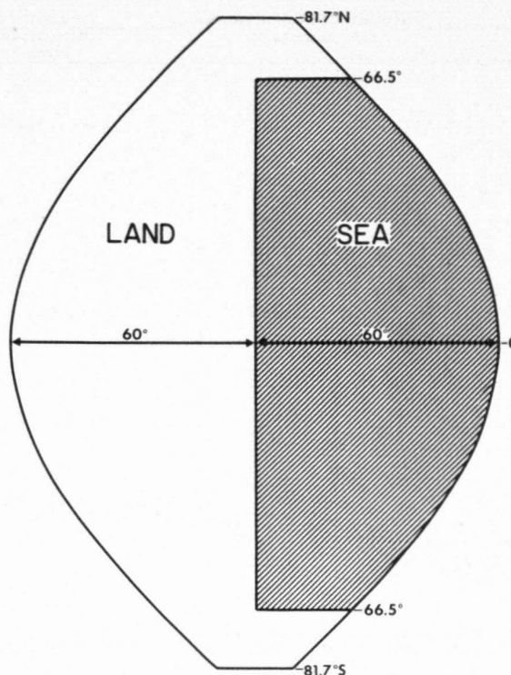
FIGURE 1.—Distribution of the continents and the ocean in the ocean-atmosphere model. Cyclic continuity is assumed at the eastern and western ends of the domain.
