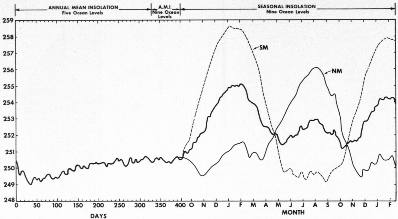
FIGURE 2.—Time variation of atmospheric potential energy ( 10^9 \text{ J} \cdot \text{cm}^{-2} ) for the entire period of the time integration of the joint ocean-atmosphere model. The total potential energy is represented by a solid heavy line, the Northern Hemisphere mean potential energy (NM) by a thin solid line, and the Southern Hemisphere mean potential energy (SM) by a thin dashed line.
