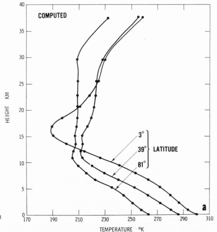
FIGURE 5.—The observed annual mean temperature profiles of Starr and collaborators for three different latitudes are compared with corresponding computed profiles.
