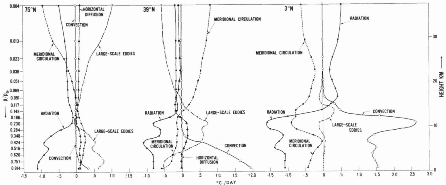
FIGURE 17.—The vertical distribution of the various heat balance components at three different latitudes. (Units: ^{\circ}\text{C}/\text{day} .)
