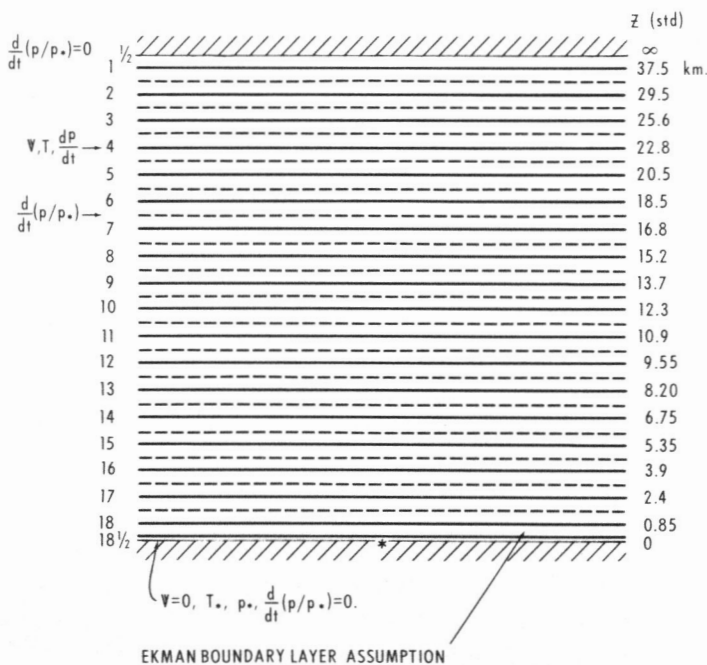
FIGURE 1.—The Q levels used in the model and their approximate heights. The levels at which the model variables are predicted are indicated.
