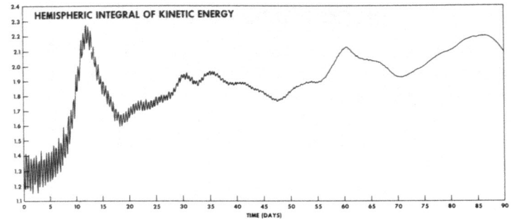
FIGURE 2.—Time variation of the hemispheric integral of kinetic energy illustrating the instability produced by the initial conditions and its subsequent damping. (Units: 10^2 joule.)
