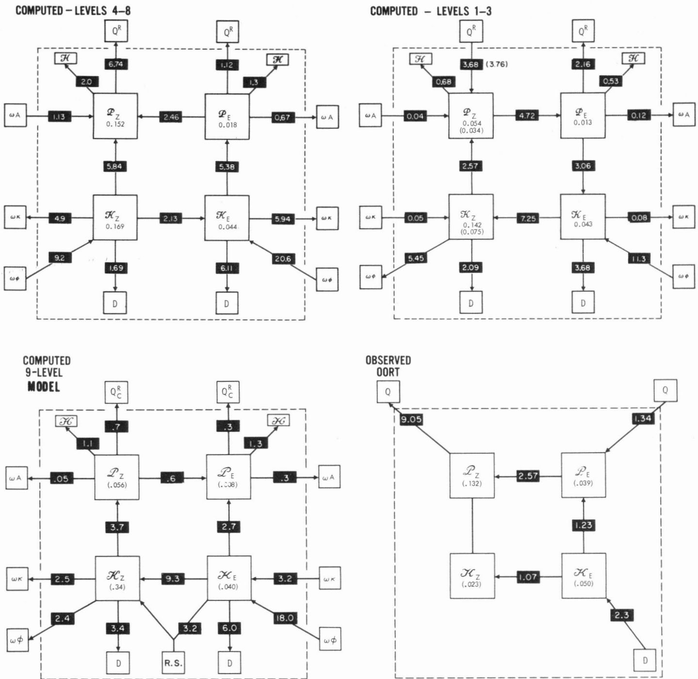
FIGURE 24.—Four box energy diagrams of the stratosphere. The upper part of the figure gives the results for the middle stratosphere (levels 1-3, 0-23.4 mb.) and the lower stratosphere (levels 4-8, 36-117 mb.) of the present model. In the lower part the corresponding results are given for the lower stratosphere (34-126 mb.) of the 9-level model and for the actual atmosphere (30-100 mb.). The energy exchange with the other layers of the atmosphere is shown by the arrows extending outside the domain enclosed by the dashed line. R.S. in the 9-level model gives the mass integral of the Reynolds stress term. The unit of energy transformation is (10^{-3} \text{ joule cm.}^{-2} \text{ mb.}^{-1} \text{ day}^{-1}) , and the unit of energy is \text{joule cm.}^{-2} \text{ mb.}^{-1}
