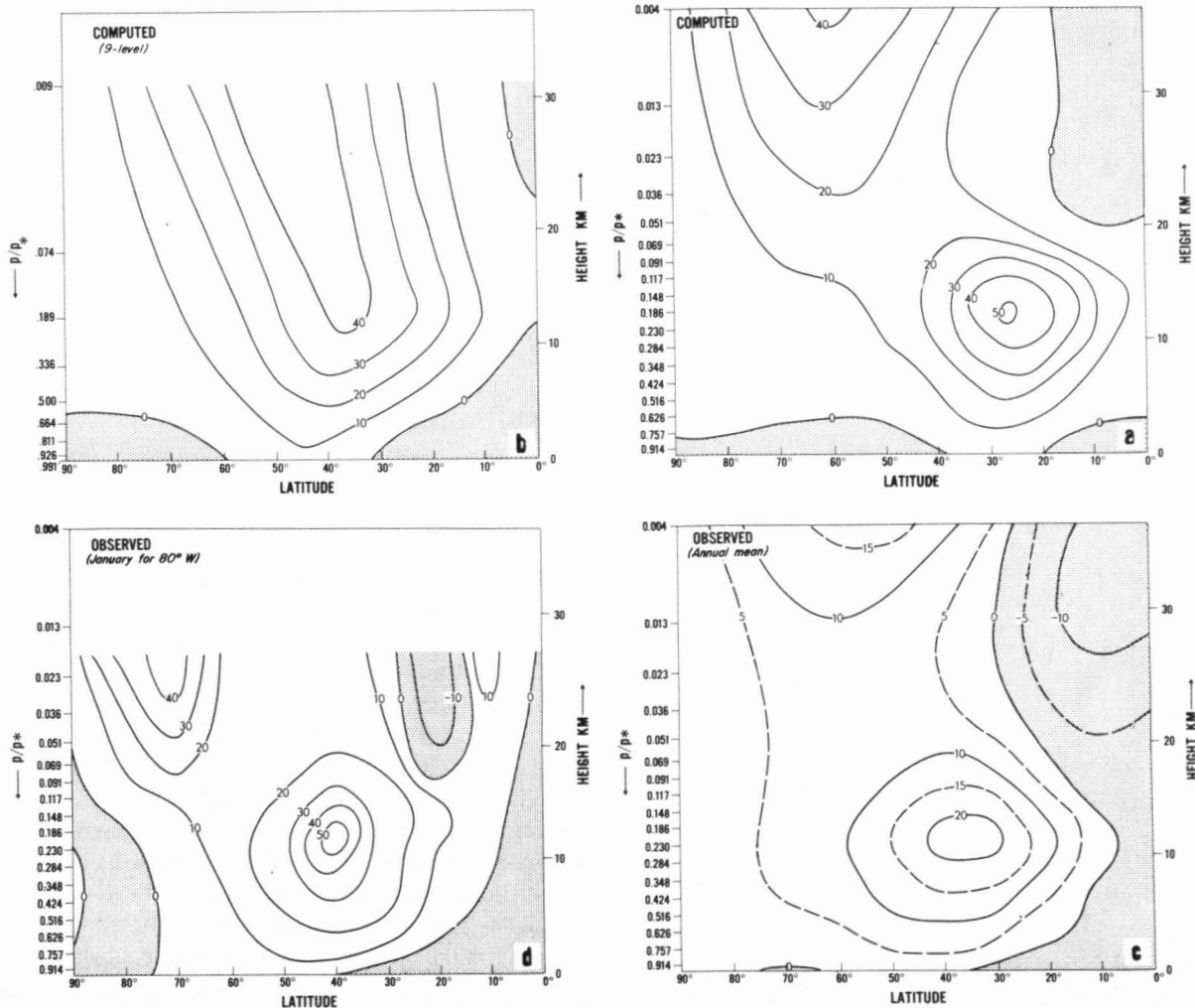
FIGURE 6.—The latitude-height distribution of the zonal mean zonal wind. In the upper half of the figure winds computed by the 18- and 9-level models are shown on the right and left respectively. In the lower half observed annual mean winds (principally Starr and collaborators) and also winds at 80°W. for January (Kochanski [11]) are given for comparison. Shaded areas are regions of easterly winds. (Units: m./sec.)
