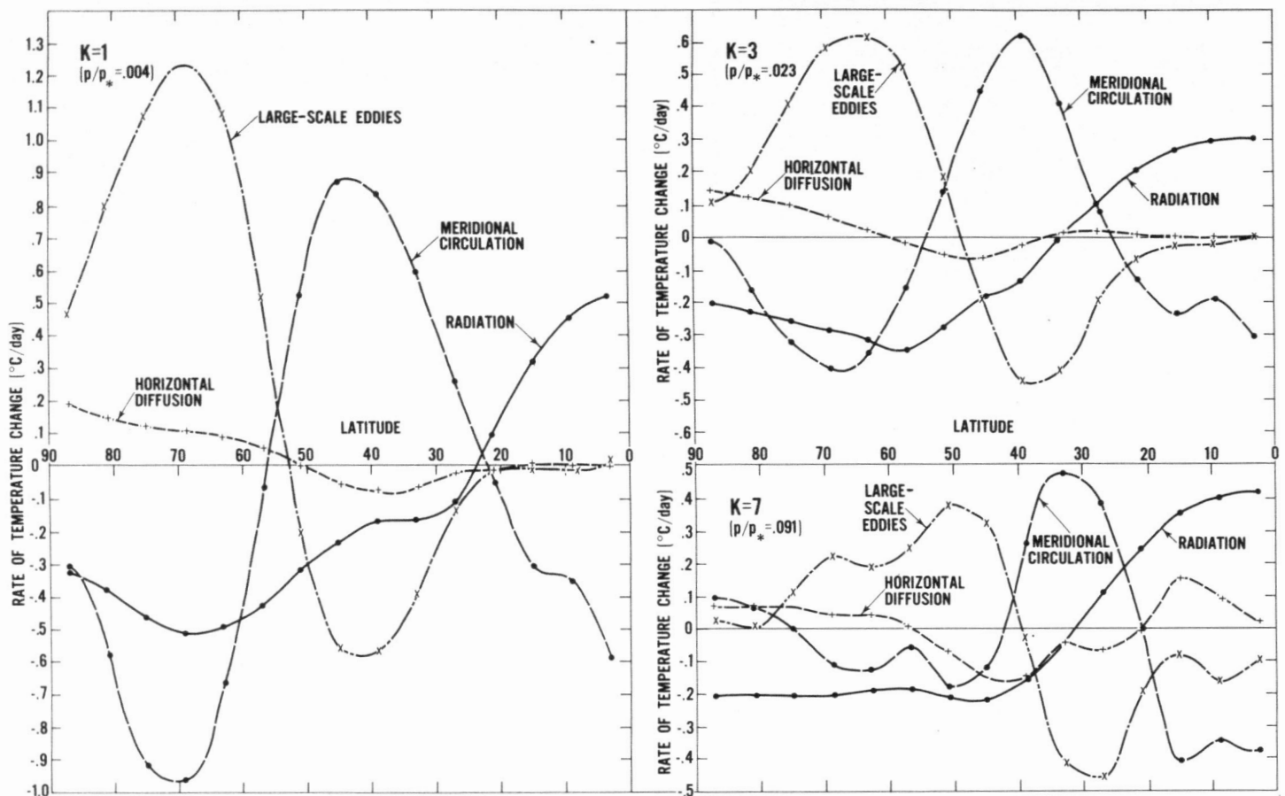
FIGURE 19.—The variation with latitude of the various heat balance components at different heights in the stratosphere.
