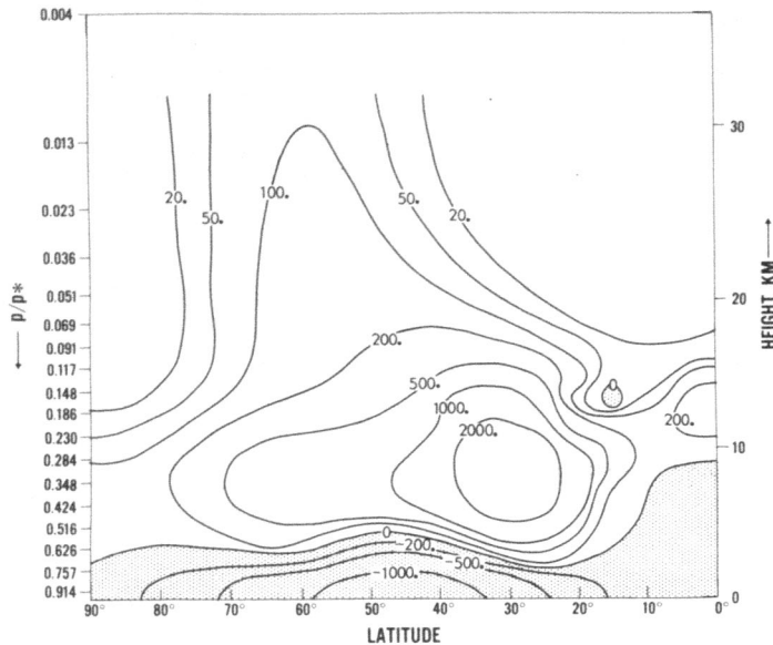
FIGURE 22.—The latitude-height distribution of the vertical flux of geopotential height -\omega'\phi' due to the large-scale eddies. Shaded areas are regions of downwards flux. (Units: ergs cm. -2 sec. -1 )
