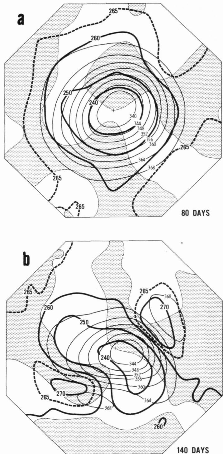
FIGURE 26.—The hemispheric variation of temperature (thick isolines), meridional velocity, and geopotential height (thin isolines) for the top level of the model at two different times illustrating the changes produced by the forcing from below. S areas are regions of northwards velocity. (Units: temperature, °K.; geopotential height, 100 m.)
