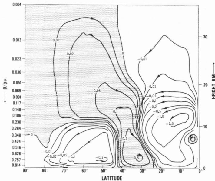
FIGURE 9.—The stream function illustrating the meridional cell structure of the model atmosphere. (Units: sec. -1 )
