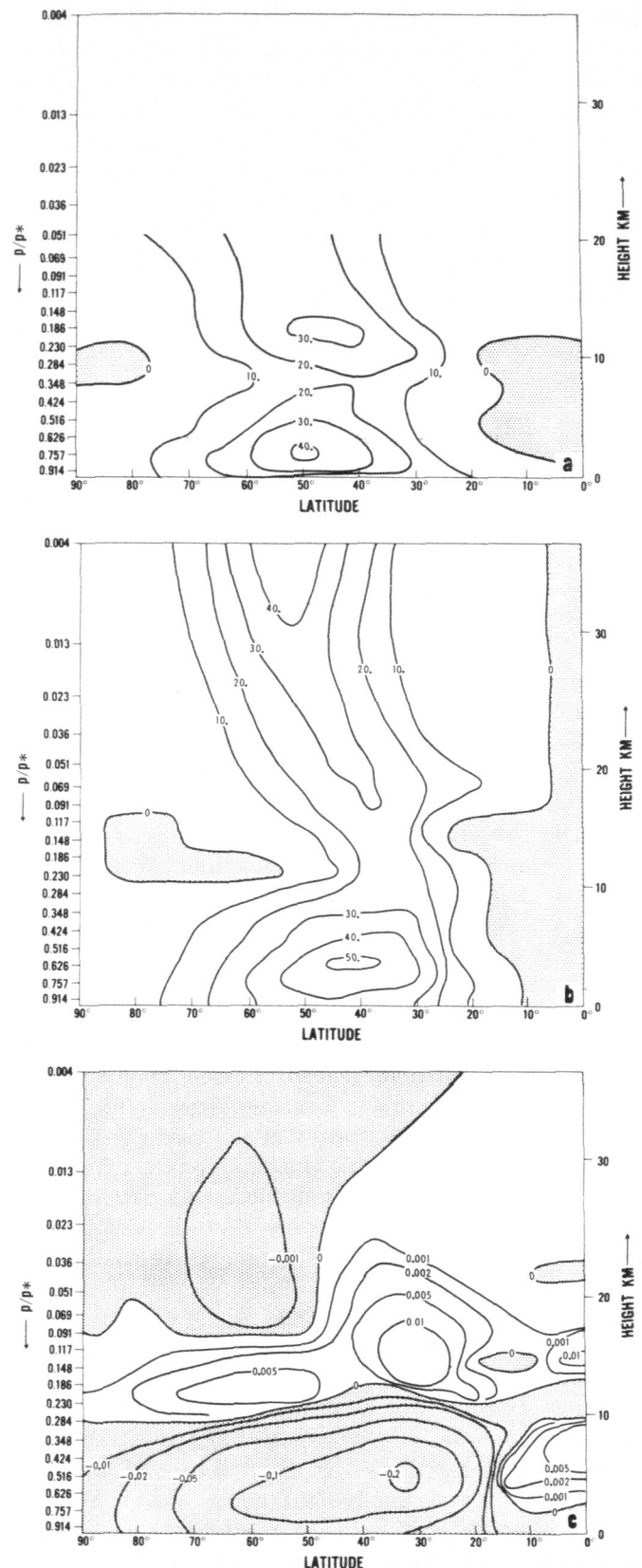
FIGURE 13.—The latitude-height distribution of the northward flux of heat by large-scale eddies (units: 10^{21} ergs atm. -1 sec. -1 ) for observed and computed conditions are given in the upper and middle parts of the figure respectively. The observed flux due to Starr and co-workers contains the contributions of both standing and transient eddies. In the lower part of the figure the computed vertical heat flux on the isobaric surface due to eddies is shown. Shaded areas are regions of upwards or equatorwards flow. (Units: 10^6 ergs cm. -2 sec. -1 )
