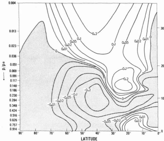
FIGURE 10.—The latitude-height distribution of the computed northward flux of angular momentum by large-scale eddies. Shaded areas are regions of equatorwards flow. (Units: 10^{27} gm. \text{cm}^2 \text{sec}^{-2} \text{atm}^{-1} )
