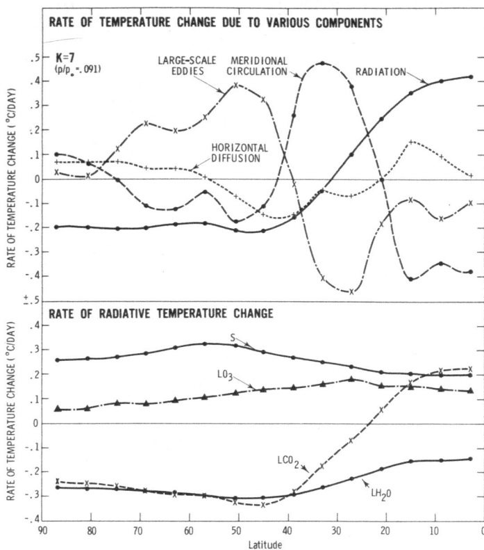
FIGURE 18.—The variation with latitude in the lower stratosphere of the various heat balance components. For further explanation refer to the caption of figure 16.
