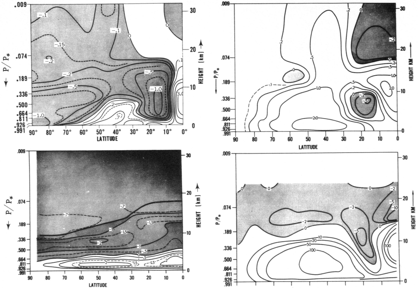
FIGURE 12C4.—Latitude-height distributions of the northward transport of heat ( 10^{17} joule \text{mb.}^{-1} \text{day}^{-1} ) and that of the upward transport of heat ( \text{joule cm.}^{-2} \text{day}^{-1} ) by the large-scale eddies are shown in the upper and lower part, respectively.
