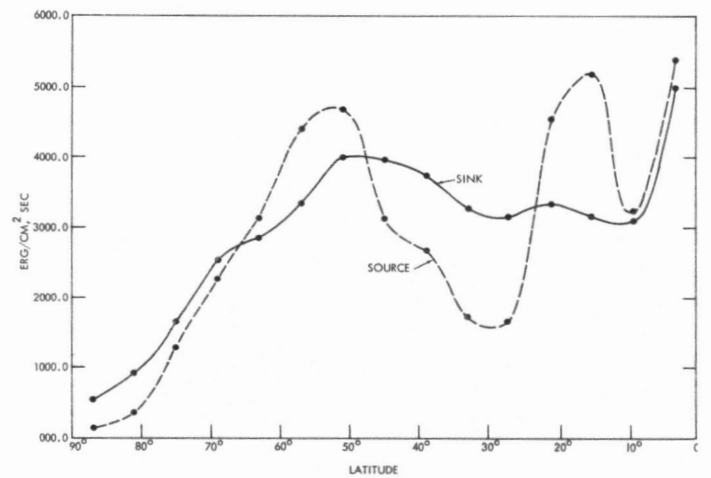
FIGURE 9.4.—The latitudinal distributions of source ( -\mathbf{V} \cdot \nabla \phi ) and sink ( \mathbf{V} \cdot \mathbf{F} ) of kinetic energy in the model atmosphere.
