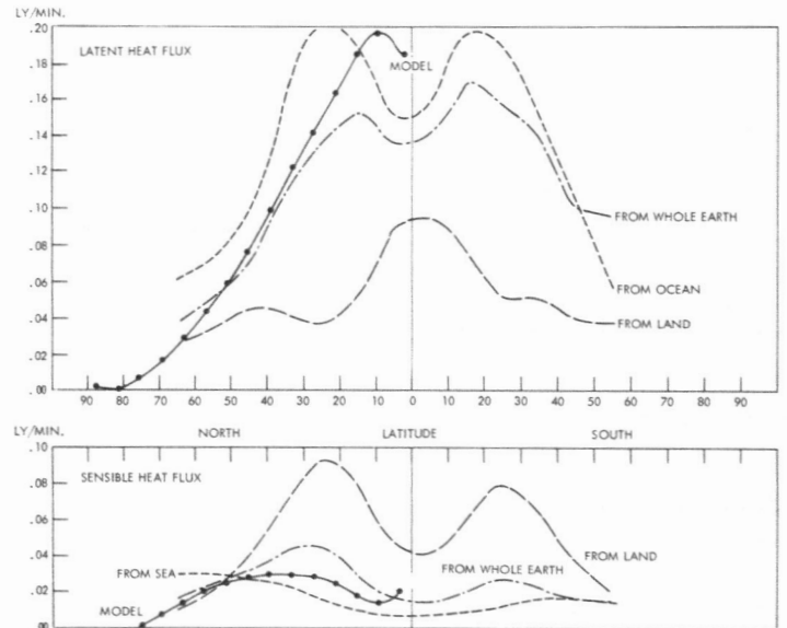
FIGURE 11.2.—Latitudinal distributions of latent and sensible heat flux from the earth to the atmosphere. The distributions, which were obtained by Budyko [5] for land, sea, and the whole earth, are compared with the distributions obtained from our model.
