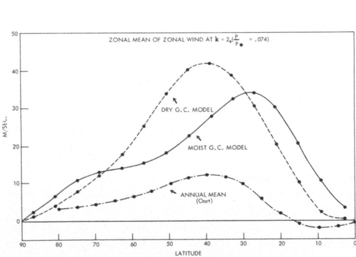
FIGURE 6.2.—Latitudinal distribution of the zonal mean of the zonal wind at the 2d model level ( P/P^* = 0.074 ) are shown together with that at the 75-mb. level of the actual atmosphere obtained from the results of Oort [24].
