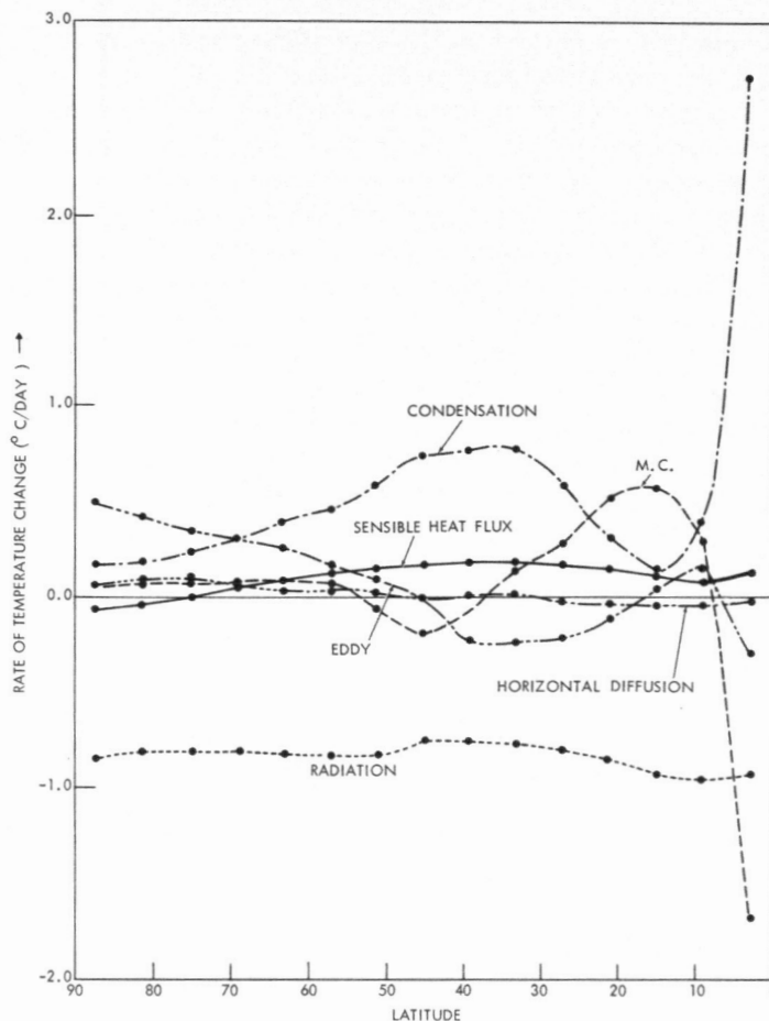
FIGURE 12B7.—The latitudinal distributions of the rate of temperature change in the model atmosphere by condensation, radiation, sensible heat flux from the earth's surface, the meridional circulation (M.C.), the large-scale eddies (EDDY), and horizontal subgrid-scale mixing (HORIZONTAL DIFFUSION).
