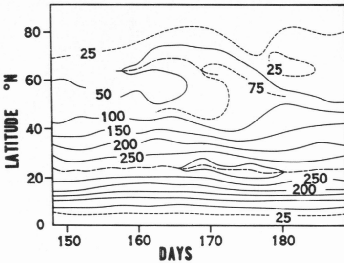
FIGURE 9.1.—The variation of the latitudinal distribution of zonal kinetic energy with time. Unit is joule cm. -2
