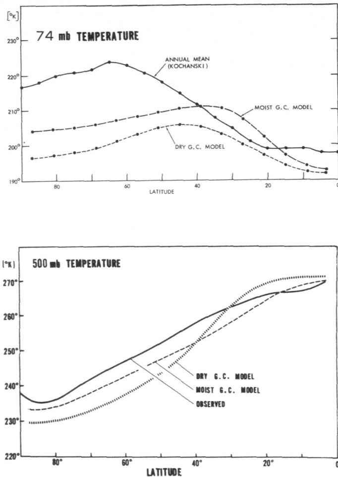
FIGURE 5.3—The latitudinal distribution of observed annual mean temperature and computed temperature at different levels of the atmosphere. The observed distributions at the 74-mb. and at the 500-mb. levels are obtained from the results of Kochanski [13] and Peixoto [26] respectively.
