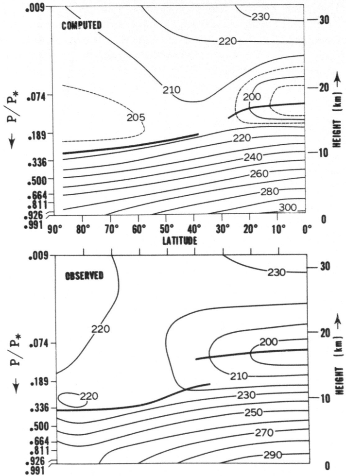
FIGURE 5.1.—In the upper and lower part, the latitude-height distribution of temperature of the model atmosphere and that of the actual atmosphere (Peixoto [26], Oort [24], and Kochanski [13]), are shown respectively.
