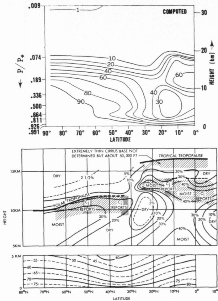
FIGURE 7.3.—In the upper part of the figure, the latitude-height distribution of relative humidity (in percent) of the model atmosphere is shown. In the lower part is shown that of the actual atmosphere for summer season (by Murgatroyd [21], Telegadas and London [39]).
