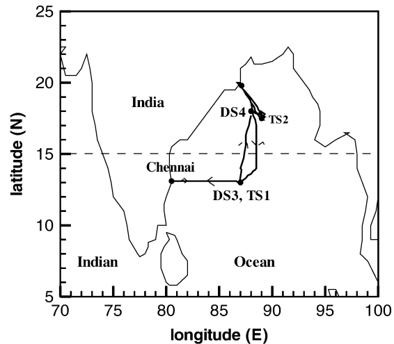
FIG. 2. Moored buoy locations and ship time series at observation stations (TS1 and TS2) in the Bay of Bengal during BOBMEX. Buoy in the head of the bay is located at DS4 (18°N, 88°E) and in the central bay at DS3 (13°N, 87°E). TS1: 13°N, 87°E; TS2: 17.5°N, 89°E.
