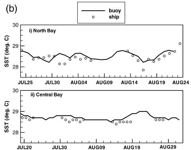
FIG. 3b. Variation of the daily average SST from the buoy and ship in (i) the north bay and (ii) central bay.
