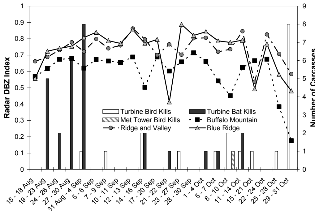
Figure 6-4. Averaged NEXRAD radar results at Buffalo Mountain, Ridge and Valley, and Blue Ridge sites and number of bird and bat fatalities at Buffalo Mountain. Horizontal axes show the time intervals between carcass searches. A) Spring 2001. B) Fall 2001. C) Spring 2002. D) Fall 2002.
