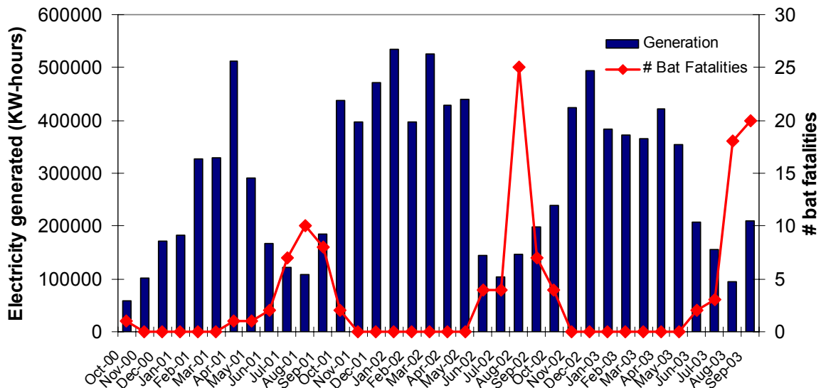
Figure 6-7. Monthly windfarm generation and number of bat fatalities found at the Buffalo Mountain Windfarm.
