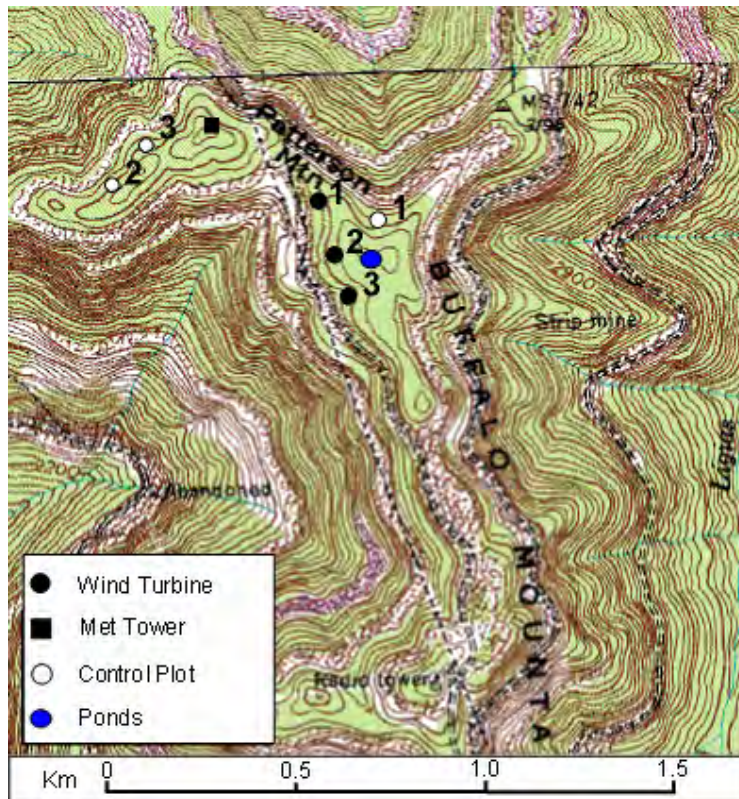
Figure 4-1. Configuration of Buffalo Mountain Windfarm, 2000-2003, showing locations of turbines, meteorological tower, control plots, and ponds.
