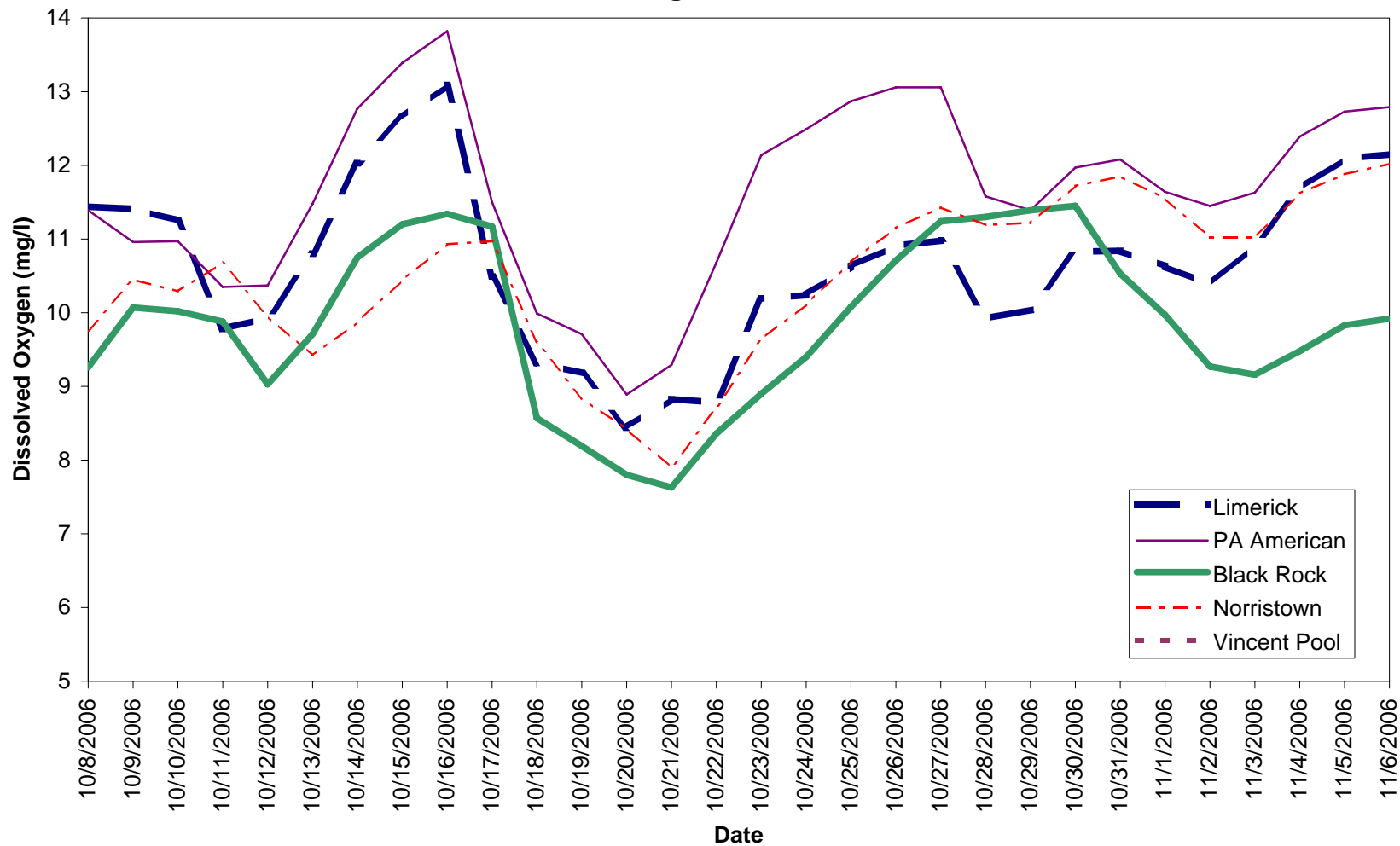
Mean Daily Schuylkill River Dissolved Oxygen October 8 through November 6 2006
