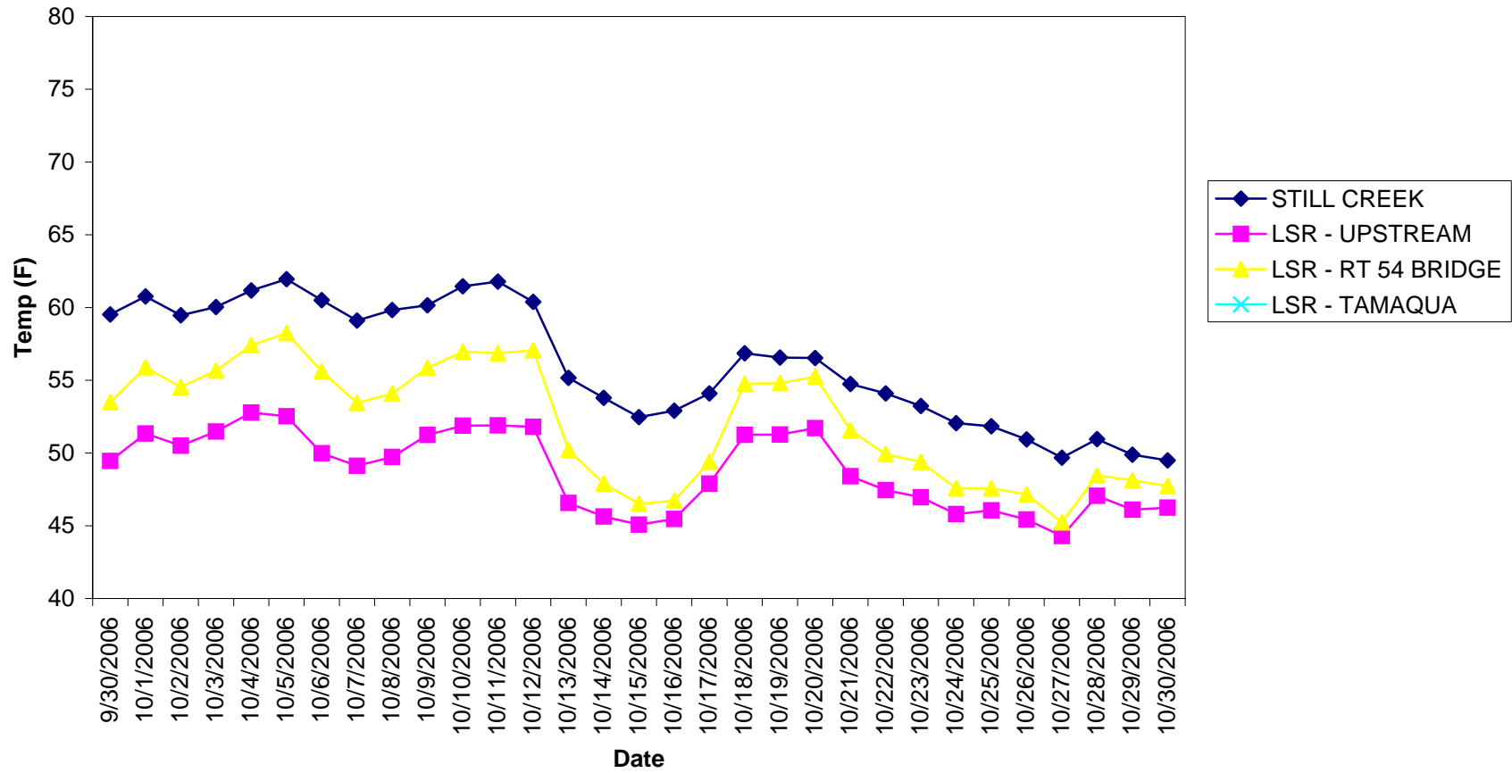
Still Creek & Little Schuylkill River Daily Average Temperatures October 2006
