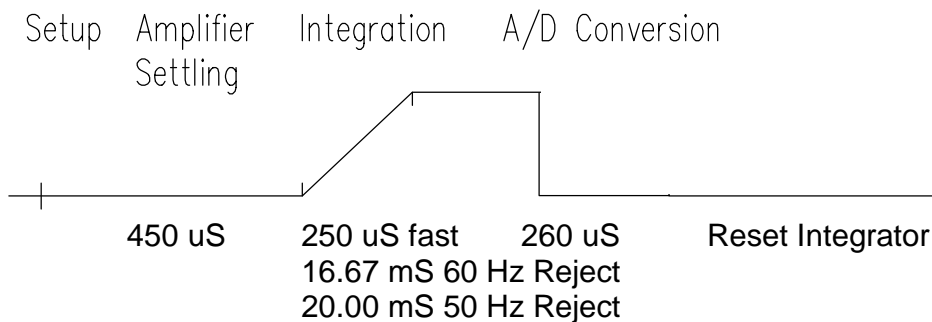
FIGURE 13.1-2. Timing of Single-Ended Measurement
