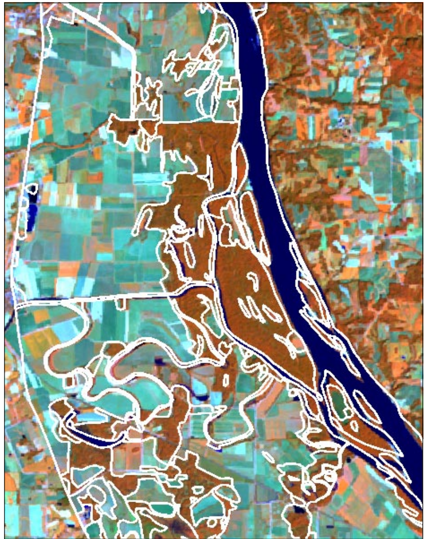
Figure. The River Engineering and Environmental Geospatial Information System (REEGIS) land cover linework for the Whitney quadrangle of the Open River displayed over a Landsat Thematic Mapper satellite image.
