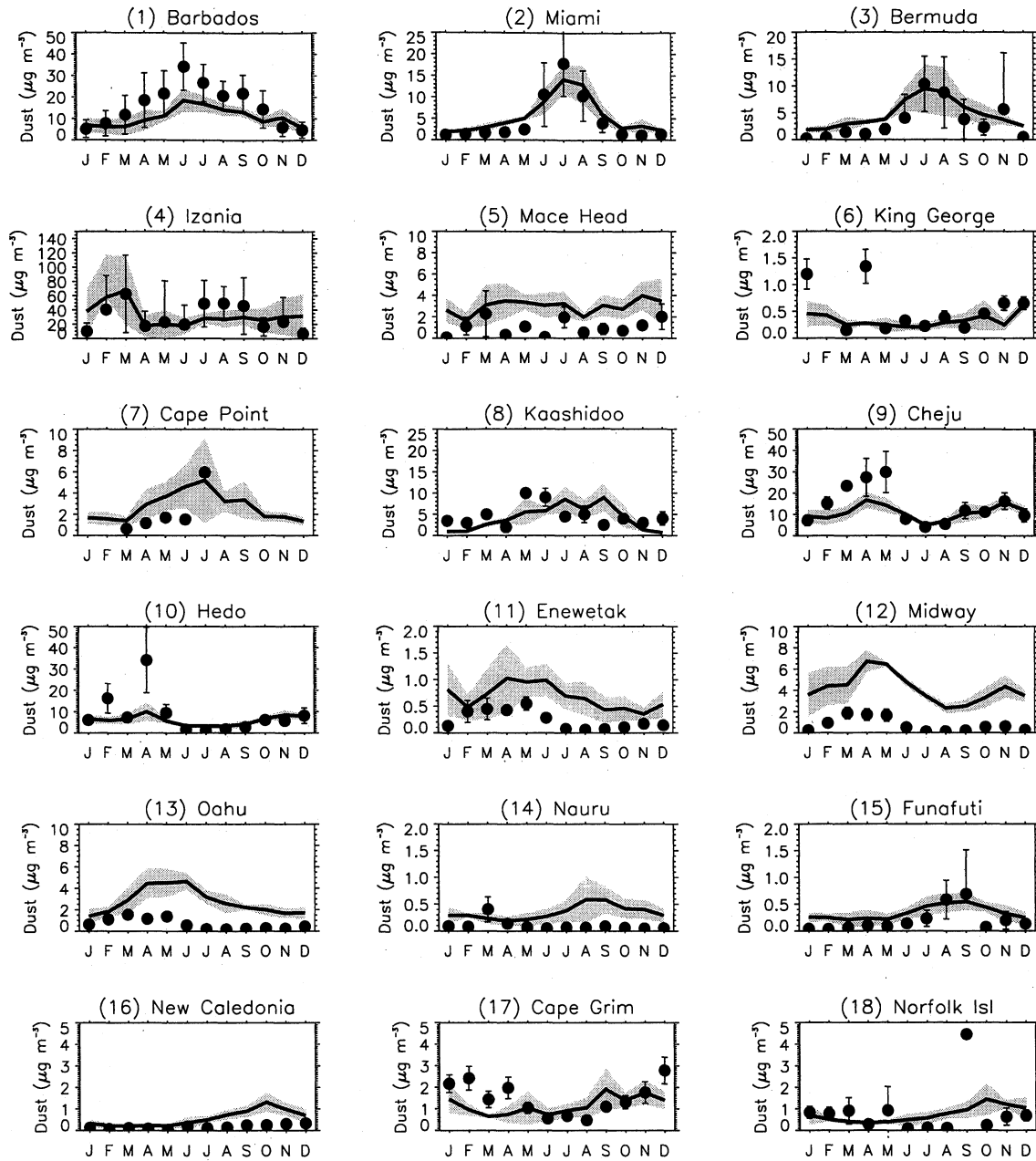
Figure 4. Comparison of monthly dust concentration, simulated and observed at 18 sites, in units of \mu\text{g m}^{-3} .
