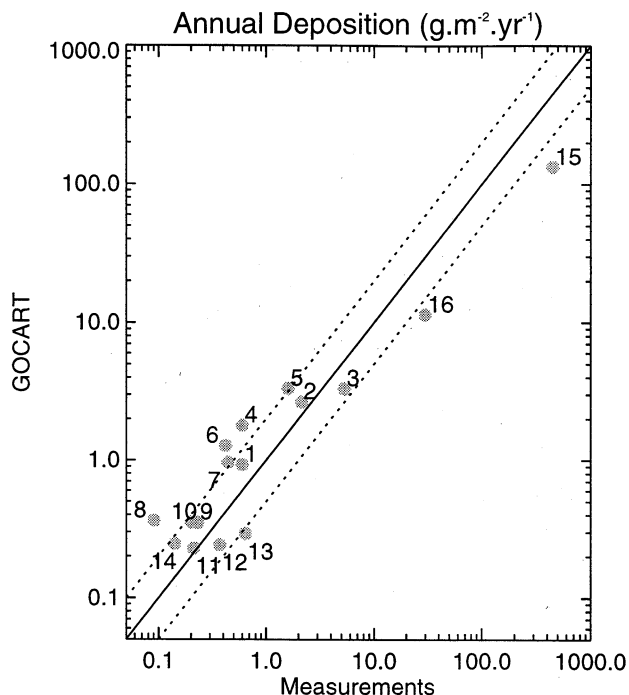
Figure 7. Comparison of annual total deposition flux simulated and observed at 16 sites.
