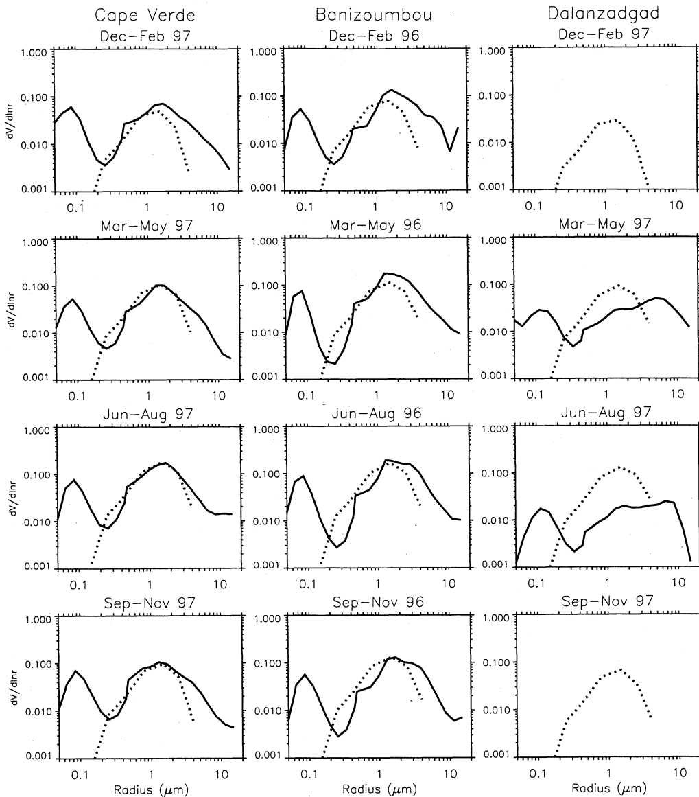
Figure 11. Comparison of volume size distribution ( \mu\text{m}^3 \mu\text{m}^{-2} ) simulated (dashed line) and retrieved (continuous line) from AERONET data.
