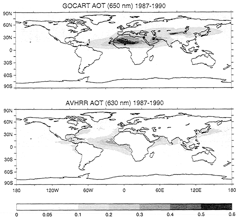
Figure 8. Comparison of the mean optical thicknesses (top) simulated at 650 nm and (bottom) observed at 630 nm by AVHRR from 1987 to 1990.
