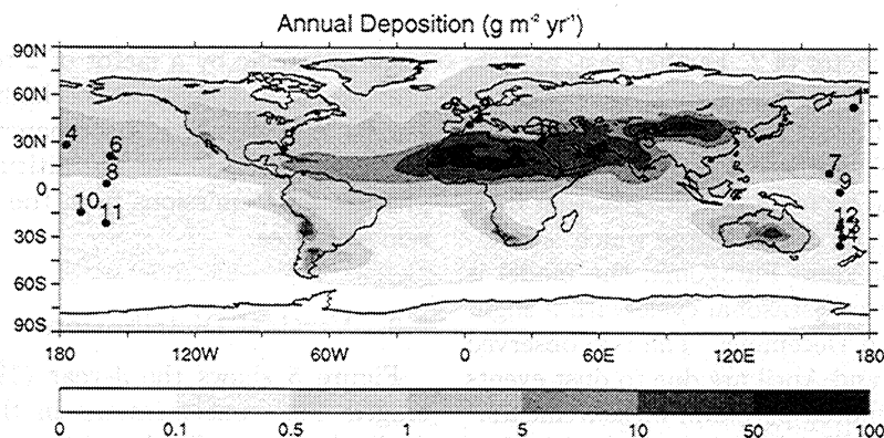
Figure 6. Global distribution of the annual total deposition flux ( \text{g m}^{-2} \text{yr}^{-1} ), averaged over 5 years simulation (1987-1990 and 1996).
