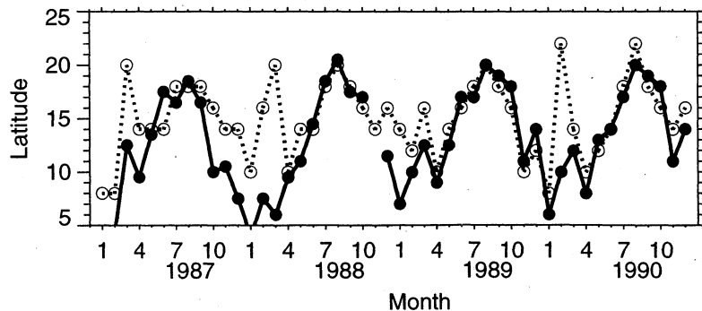
Figure 9. Latitudinal variation of the maximum optical thickness along the 25°W meridian deduced from AVHRR data (continuous line) between January 1987 and December 1990 (November 1988 is missing), and from the model simulations (dashed line).
