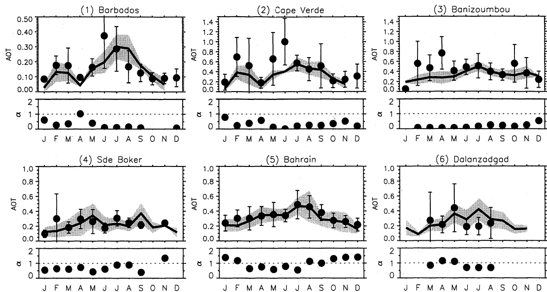
Figure 10. Comparison of optical thicknesses simulated (bold line) and measured by AERONET (dots) at six sites; the standard deviation of the simulated and observed values are represented by shading and vertical segments, respectively. The lower panels give the monthly Angstrom parameter \alpha , calculated from the AERONET optical thicknesses at 440 and 670 nm.
