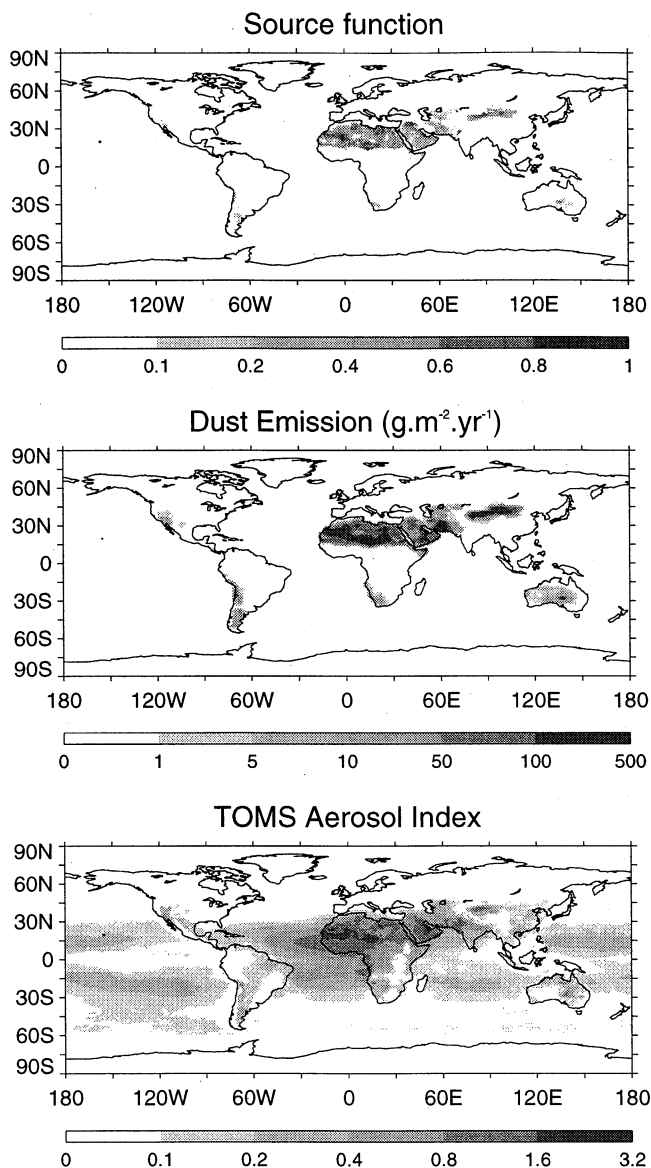
Figure 1. Comparison between (top) the dust source function, and (middle) the dust emission and (bottom) distributions of TOMS aerosol index. The dust emission and TOMS aerosol index are average values from 1987 to 1990.
