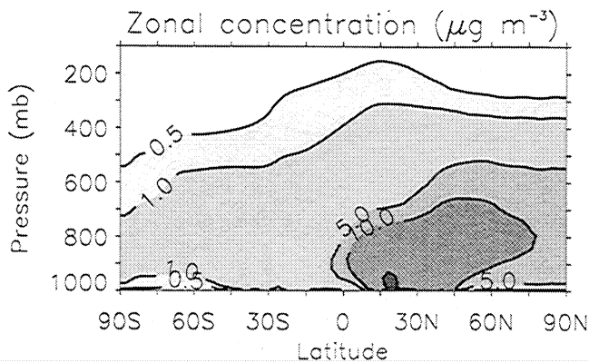
Figure 5. Zonal mean dust concentration with isolines at 0.5, 1, 5, 10, and 50 \mu\text{g m}^{-3} .
