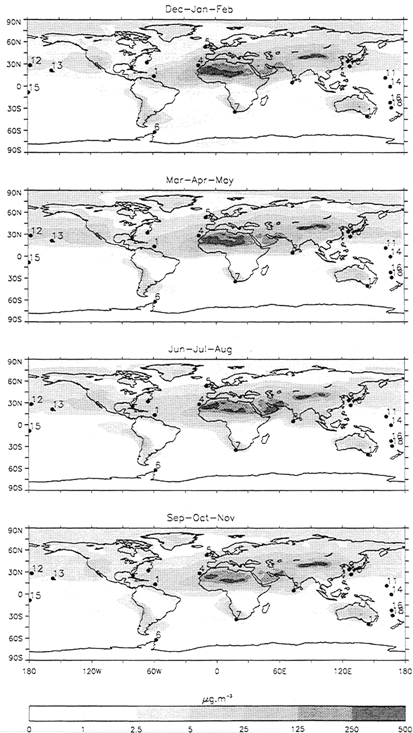
Figure 2. Seasonal variation of dust concentration, averaged over 5 years (1987-1990 and 1996), in units of \mu\text{g m}^{-3} .
