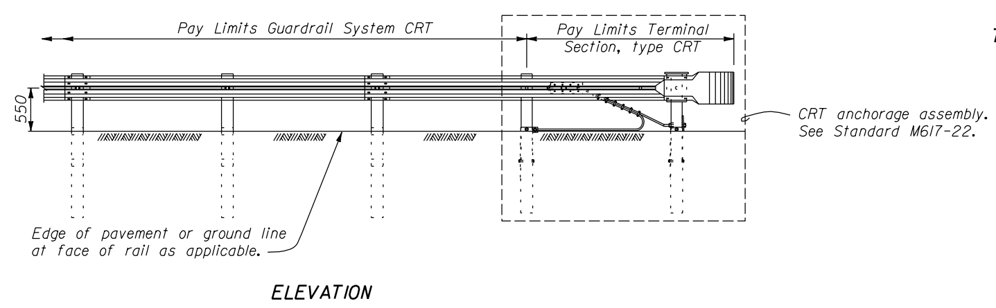
GUARDRAIL SYSTEM CRT WITH CABLE RELEASING TERMINAL CRT POSTS
