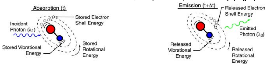
Figure 1: Schematic illustration of laser induced fluorescence. A photon of wavelength (color) \lambda_1 excites an electron to a higher energy state. When the electron returns to its original state it emits light of wavelength \lambda_2 . The emission intensity is linked to temperature and concentration of the molecules. The color of the absorbed and emitted light is specific for each type of molecule, thus finger-printing at a molecular level is enabled.
